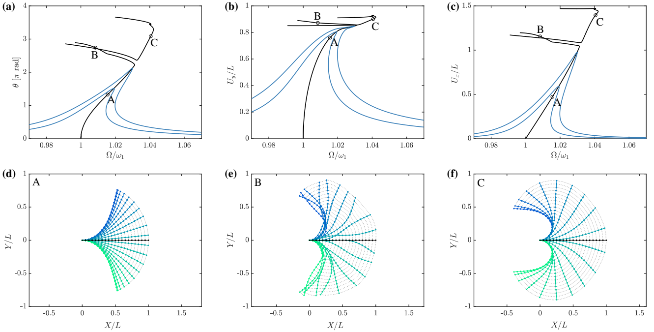
Fig. 4 First vibration mode of the cantilever beam of Fig. 3(a). Top row: forced responses ( \hat{F}_0 = 0.05 and \hat{F}_0 = 0.08 ) and backbone curve of (a) the cross-section rotation \theta , (b) the scaled transverse displacement U_y/L , (c) the scaled axial displacement U_x/L at the tip of the cantilever. Maximum amplitude over one period of oscillation. Bottom row: nonlinear deformed shape at (a) low amplitude (point A), (b) internal resonance (point B) and (c) high amplitude (point C); 20 snapshots per half period.
