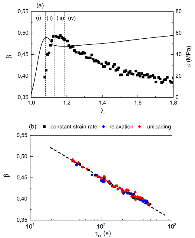
FIG. 4. (a) Stretching parameter \beta (Left axis, dots) and nominal stress \sigma (Right axis, solid line) at \dot{\lambda} = 2.5 \times 10^{-4} \text{ s}^{-1} as function of strain. (b) Relation between \beta and \tau_\alpha observed for different protocols: The constant strain rate protocol at \dot{\lambda} = 2.5 \times 10^{-4} \text{ s}^{-1} . The relaxation protocol discussed in Sec.III.2 with \lambda_w = 1.2 , t_w = 1h and \dot{\lambda} = 2.5 \times 10^{-4} \text{ s}^{-1} . The unloading protocol of Sec.III.3 with \lambda_p = 1.25 , \lambda_w = 1.2 , t_w = 1h and \dot{\lambda} = 2.5 \times 10^{-4} \text{ s}^{-1} . Note the log scale for the x-axis.
