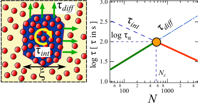
FIG. 11. Left: A slow (high density) subunit of size \xi \sim 3 - 5 nm within a faster (lower density) surrounding may relax either by internal free volume reorganization (time \tau_{int} ) or diffusion (time \tau_{diff} ) (density differences are exaggerated). Right: variation of \tau_{int} \sim N^{-1/2} (dashed curve) and \tau_{diff} \sim N^{2/3} (dash-dotted curve) vs the number N of monomers in subunits.
