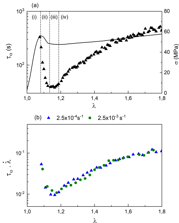
FIG. 3. (a) Mean relaxation time \tau_\alpha (Left axis, dots) and nominal stress \sigma (Right axis, line) as function of strain for \dot{\lambda} = 2.5 \times 10^{-4} \text{ s}^{-1} . (b) Dimensionless parameter \tau_\alpha \dot{\lambda} as function of strain for the two strain rates indicated. \tau_\alpha and \beta are extracted with the dielectric strength \Delta = 0.125 . The same value of \Delta is used in the rest of the article.
