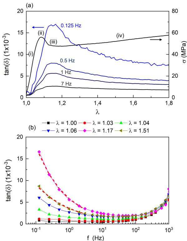
FIG. 2. (a) \tan(\delta) = -\varepsilon''/\varepsilon' (Left axis) at several frequencies \{0.125, 0.5, 1, 7\} \text{ Hz} and nominal stress \sigma (Right axis) as a function of strain for the constant strain rate protocol with \dot{\lambda} = 2.5 \times 10^{-4} \text{ s}^{-1} . (b) \tan(\delta)(f) spectra pick up at several strains. In red dashed line, results of the fit Eq.1.
