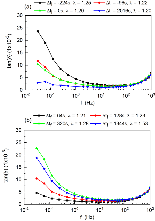
FIG. 9. Dielectric \tan(\delta)(f) spectra for the experiment Fig.8 at several strains (a) during the retraction and the pause step and (b) during the recovery step. \Delta t_i = t - t_i and \Delta t_f = t - t_f .
