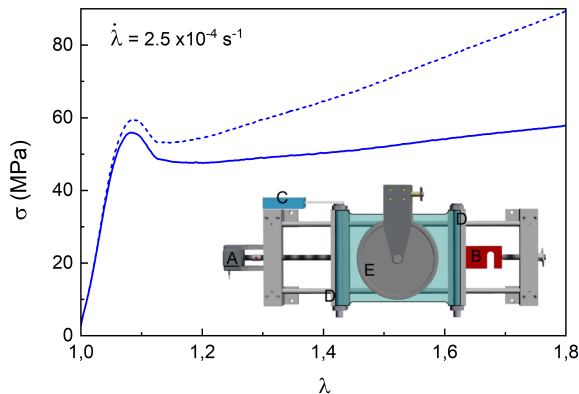
FIG. 1. Nominal stress (solid line) versus strain. An estimation of the true stress (dashed line) is also indicated, see discussion. Inset: Sketch of the experimental setup. (A) motor, (B) cell load, (C) linear actuator, (D) sample fastening cylinders, and (E) electrodes for the dielectric measurement. The all setup is protected by a Faraday cage to minimize low frequency electromagnetic perturbations coming from the outside.
