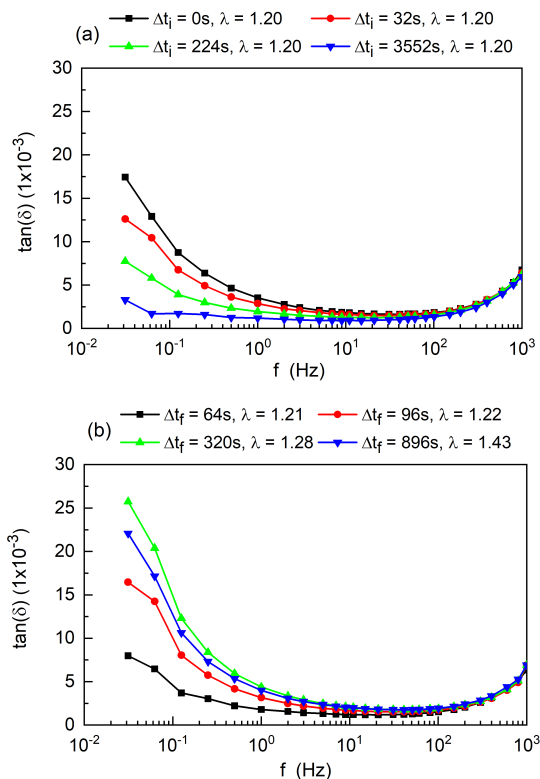
FIG. 6. Dielectric \tan(\delta)(f) spectra for the experiment Fig. 5 at several strains (a) during the pause step and (b) during the recovery step. \Delta t_i = t - t_i and \Delta t_f = t - t_f .
