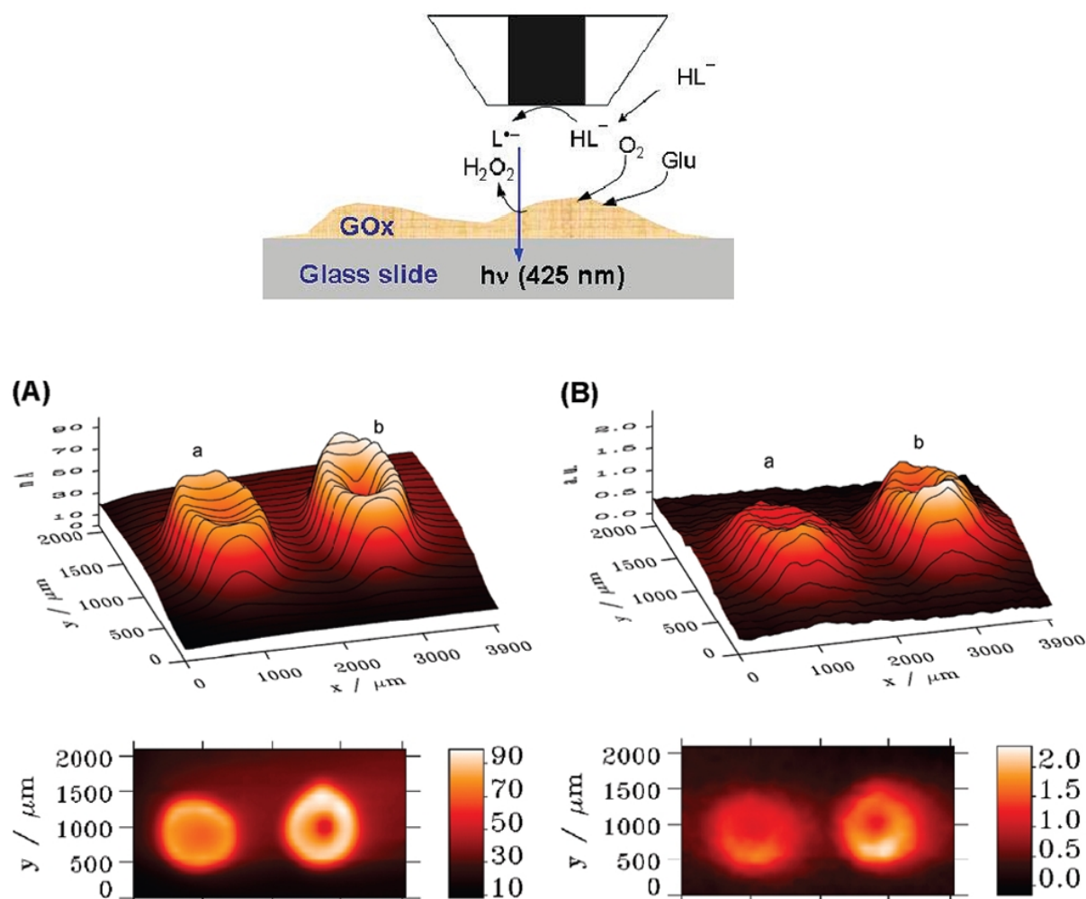
Figure 38. SECM/ECL for studying local biocatalytic activity of enzyme-polymer spots. Top: Working principle. The oxidized form of luminol ( \text{L}^{\bullet-} ) is generated at the SECM tip. When the tip is scanned over active glucose oxidase (Gox) spots light is emitted due to the reaction of oxidized luminol with \text{H}_2\text{O}_2
