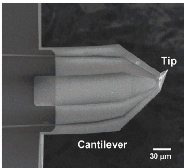
Figure 3: (a) Low- and (b) high-resolution FE-SEM images of the tip and cantilever geometry of a typical AFM-SECM probe fabricated using microfabrication and electron beam lithography. Adapted with permission from P. S. Dobson et al., Anal. Chem. 77, 424–434 (2005). Copyright 2005 American Chemical Society.
