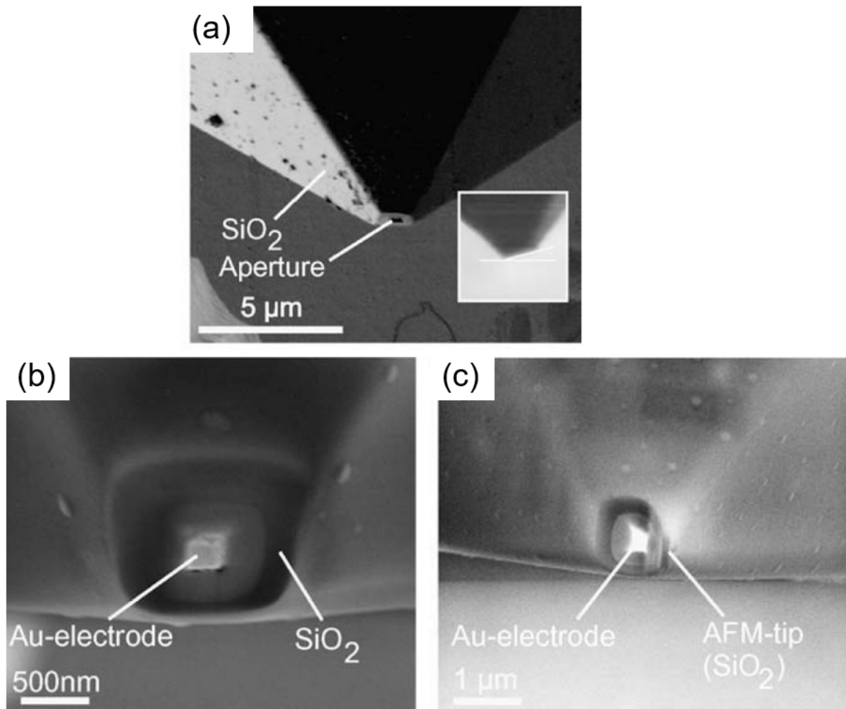
Figure 6: (a) Slice of the pyramidal tip yielding a small square electrode (inset shows the same tip at the same magnification but at a different angle in order to visualize the sloped cut of \sim 15^\circ ). (b) Electrode at the apex of the pyramid achieved by removing \text{SiO}_2 at the very tip. (c) Ion beam milling was performed so that one half of the top \text{SiO}_2 layer was left as distance holder in SECM and as AFM-tip. Reproduced with permission from M. Salomo et al., Microelectron. Eng. 87, 1537–1539 87 (2010). Copyright 2010 Elsevier B.V.
