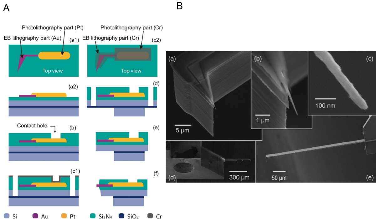
Figure 4. Left: Schematic view of the fabrication process. Top view (a1) and side view (a2) of the tip and interconnections after the lift-off process. (b) BHF etching to open the contact holes. (c1) DRIE etching through the device layer with the Cr mask which defines the chip shape. (c2) Top view of the Cr mask in step c1. (d) Backside patterned by DRIE. (e) BHF etching releases the chip. (f) KOH etching and BHF etching open the conducting tip apex. Right: SEM pictures of the fabricated probe: (a) Conductive probe. (b) Closer view of the passivation and gold tip. (c) Tip apex. (d) A bird's eye view of the chip from the handling layer. (e) 400\ \mu\text{m} \times 20\ \mu\text{m} \times 2\ \mu\text{m} cantilever with a gold conductive tip. Reproduced with permission from Y. Wu et al., Sensors Actuators A Phys. 215, 184–188 (2014). Copyright 2014 Elsevier B.V.
