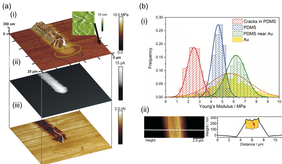
Figure 11. a) QNM-AFM-SECM measurement of a gold electrode patterned onto PDMS recorded in 2.5 mM \text{Fc}(\text{MeOH})_2 / 0.1 \text{ M KCl} . Peak force: 2 nN, amplitude: 80 nm. (i) 3D topography of the structure overlaid with the Young's modulus (calculated with a DMT fit, green mark shows increased stiffness of the PDMS surrounding the gold pattern, inset shows topography of the cracked PDMS); (ii) faradaic current image obtained with the AFM-SECM probe biased at 0.5 V vs. Ag/AgCl, and (iii) tip-sample adhesion image. b) (i) Histograms showing the different Young's modulus recorded on the patterned PDMS substrate. Cracks on the surface with 2.5 \pm 0.6 \text{ MPa} ( N=200 ) (red), the PDMS substrate with 4.6 \pm 0.5 \text{ MPa} ( N=12500 ) (blue), the PDMS near the gold structure with 6.2 \pm 0.9 \text{ MPa} ( N=4400 ) (green), and the gold structure with 5.6 \pm 1.7 \text{ MPa} ( N=2300 ) (yellow). The sputtered metal height is indicated in the profile in yellow, the red arrow indicates a gap in the center part of the structure. Reproduced with permission from P. Knittel et al., Anal. Chem. 88, 6174–6178 (2016). Copyright 2016 American Chemical Society.
