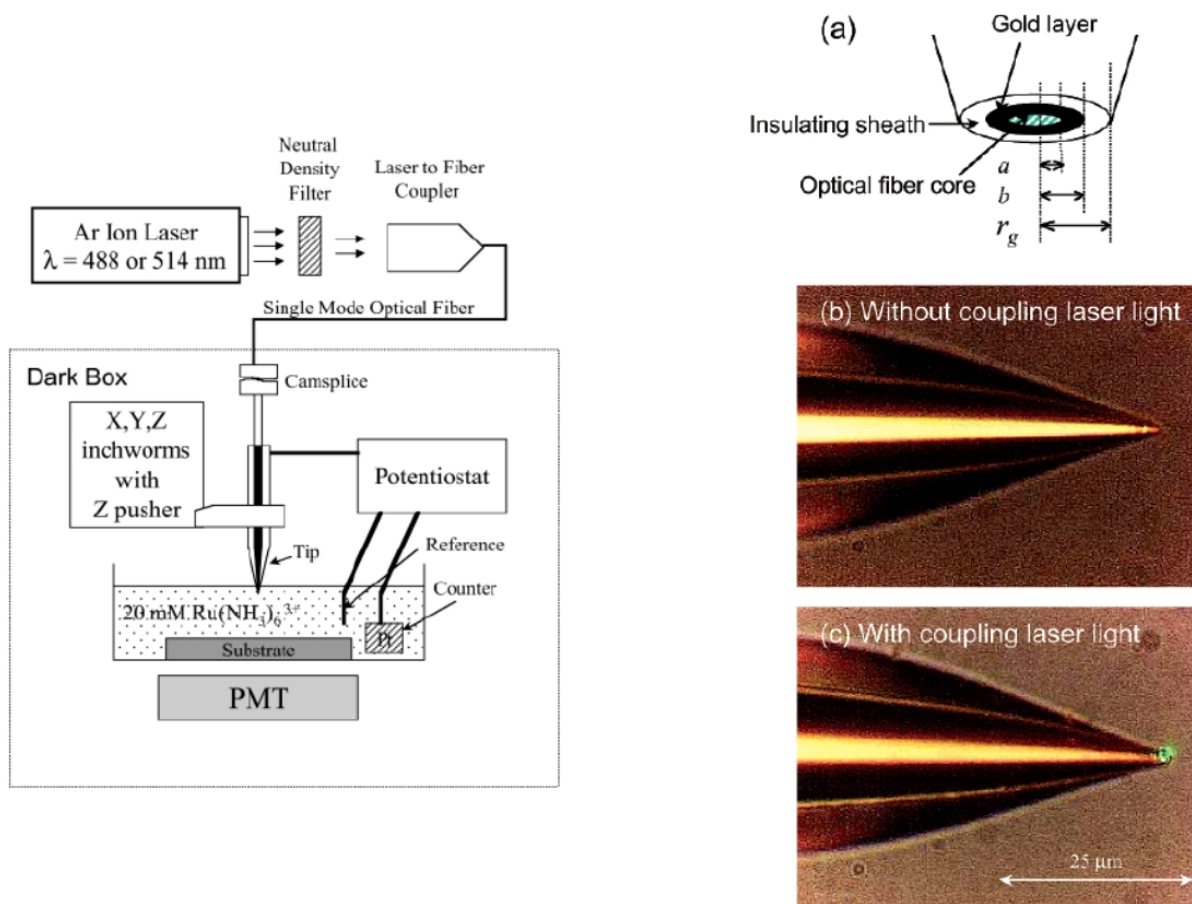
Figure 32. (Left) Block diagram of an experimental setup for combined scanning electrochemical and optical microscopy (SECM/OM). A photo multiplier tube (PMT) is positioned below the (partly transparent) substrate. (Right) (a) Schematic diagram of an ideal optical fiber/microelectrode tip for SECM/OM: A sharpened optical fiber bearing a ring-shaped microelectrode at its apex. Optical microscopy images of an anodic paint insulated combined SECM/OM tip (b) without and (c) with coupling of Ar ion laser light at 514 nm. Reproduced with permission from Y. Lee et al., Anal. Chem. 74, 3626-3633 (2002). Copyright 2002 American Chemical Society.
