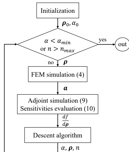
Fig. 5. Flowchart of the optimization algorithm.
