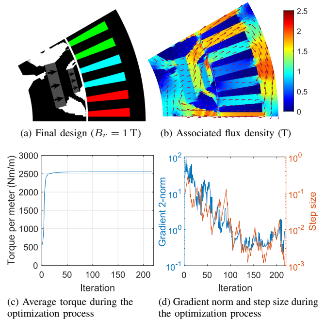
Fig. 9. Optimization results for a motor working point.
