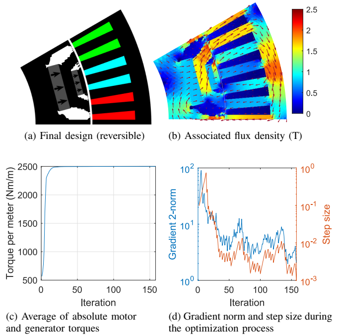
Fig. 11. Optimization results for both motor and generator working points.
