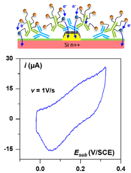
Figure S4. Cyclic voltammetry response of a monolayer of IgG/IgG-PEG-Fc immuno-assembled on a nanodot array surface whose interdot region has not been protected from non-specific adsorption by PEG-silane. 100 mM phosphate buffer pH 7.4
