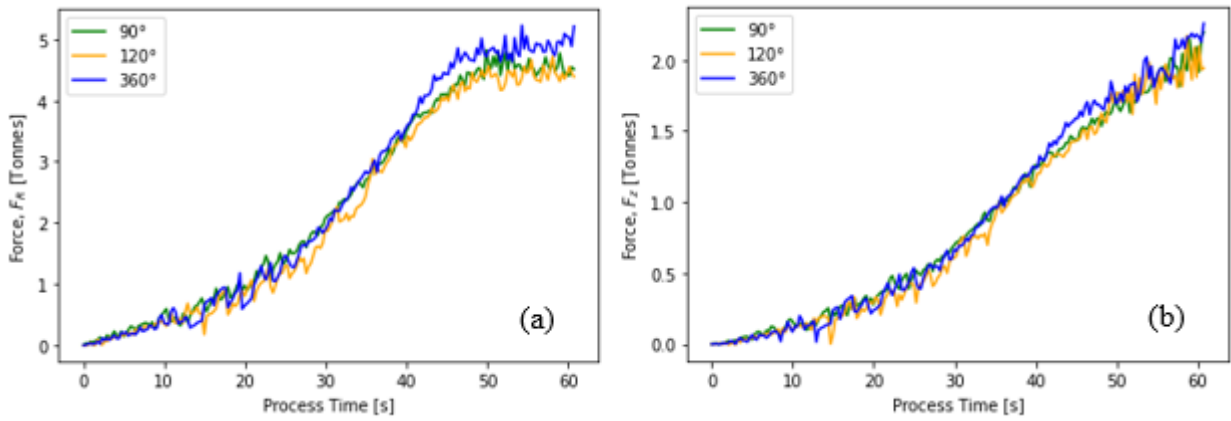
Figure 7: Roller forces in the (a) radial and (b) axial, z directions until process time of 60s
