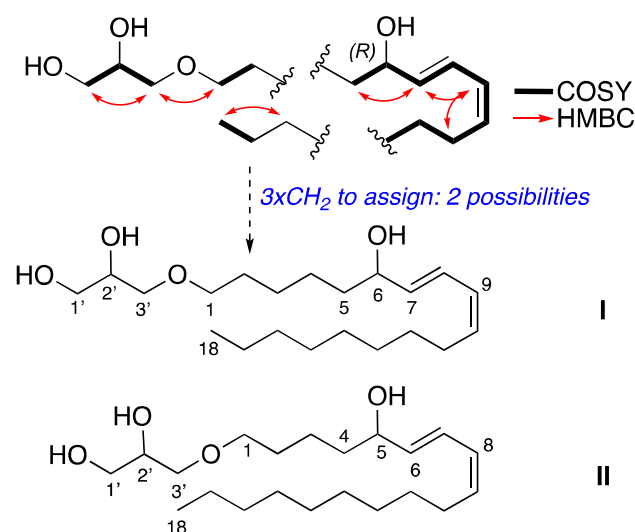
Figure 1. Fragments assigned by mass spectrometry and NMR spectroscopy and the resulting I/II structural proposals.
