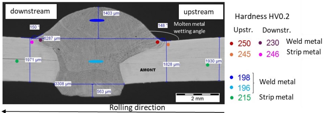
Figure 1: cross section of a real weld line after the scale-breaker. Strip metal: hot rolled AISI 304L, weld metal: filler wires ER 310 or ER 316LSi.
