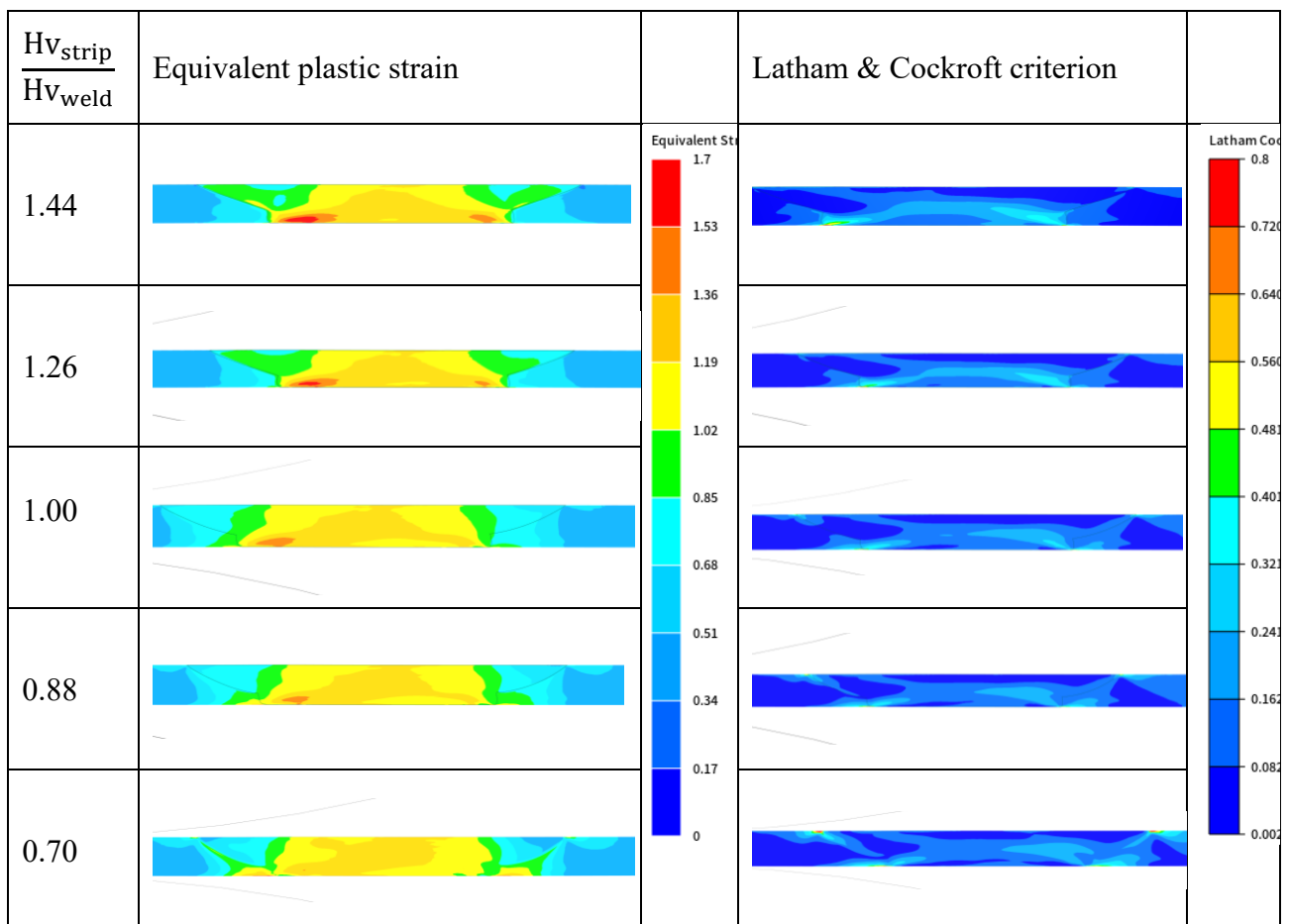
Figure 8: weld / base metal hardness ratio impact on strain and LC maps (austenitic grades). Rolling direction RD is from left to right.
