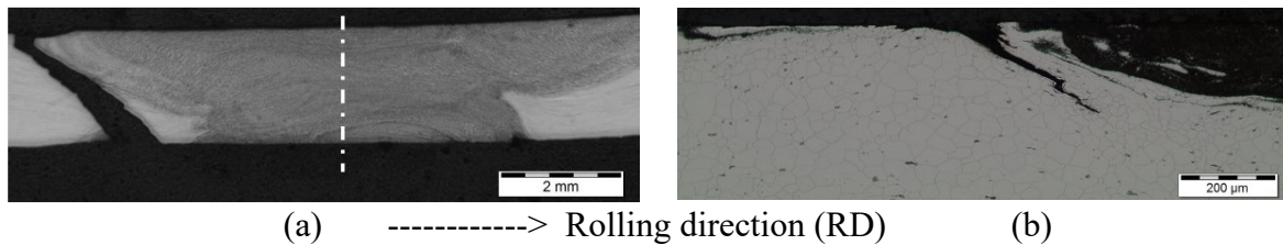
Figure 5: cross-section micrographs of fractures. (a) austenitic case ; (b) ferritic case
