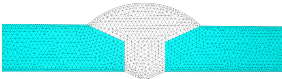
Figure 3: numerical model, geometry and meshing of the weld line and strip metal.
