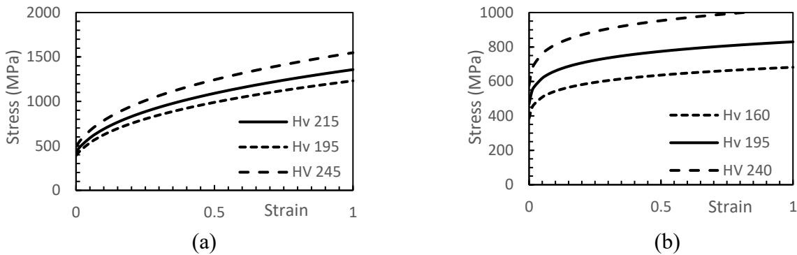
Figure 4: stress-strain curves of base metal and weld metal. (a) austenitic grade (304L); (b) ferritic grade (441). Measured curves pictured with full lines, parametric variations with broken lines.
