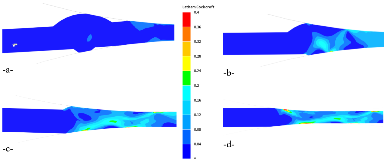
Figure 6: snake-like creeping of the bead as it enters the roll bite and progresses.
