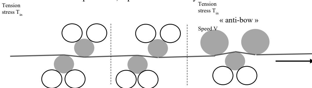
Figure 2: principle of scale-breaking by plastic bending under strip tension.
