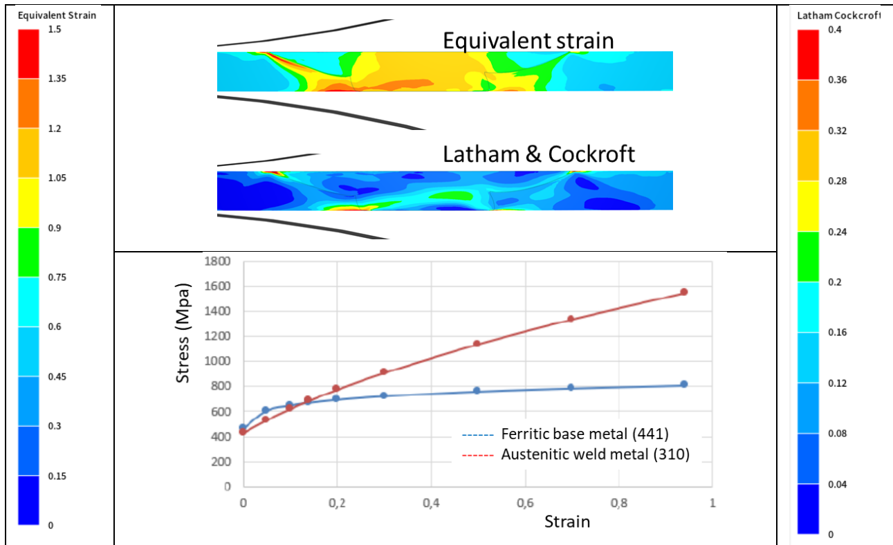
Figure 9: damage function at the exit of the roll bite, 441 ferritic steel butt-welded using ER 310.
