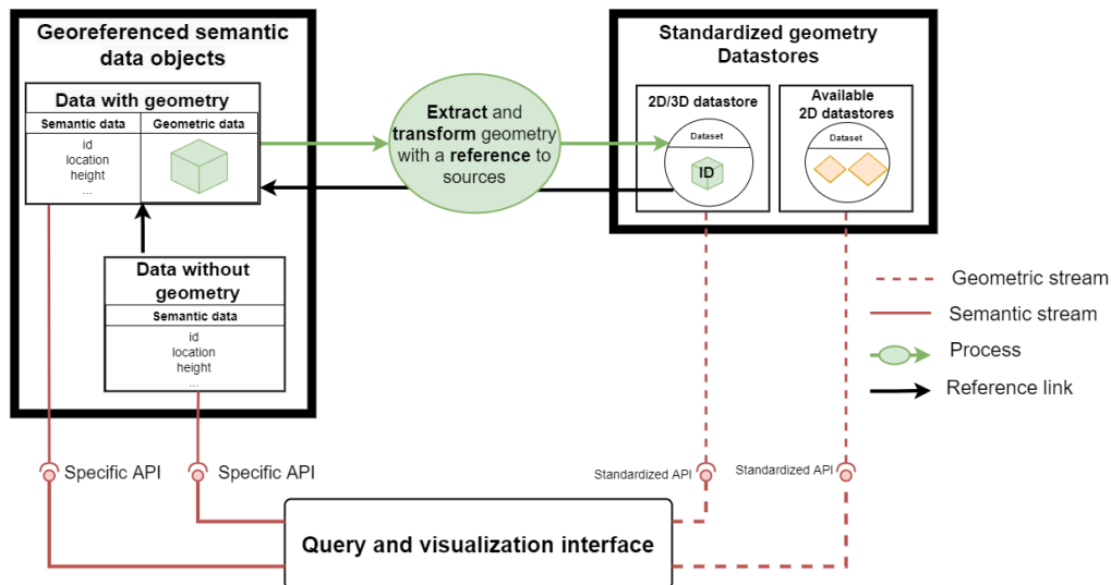
Figure 2. Logical architecture
