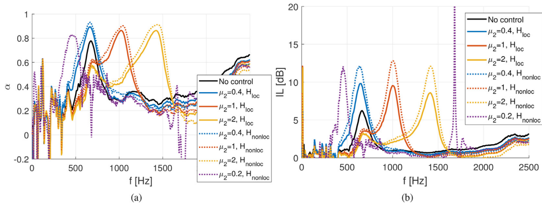
Fig. 10. Effect of the variation of the parameters of the control law ( \mu_1 = 0.4, \mu_2 = [0.2, 0.4, 1, 2] ) and target resistance ( R_{at} = 0.5\rho_0 c_0 ). Transport speed of the advection condition ( H_{nonloc} : c_a = 0.9c_0 ): a) Absorption coefficient ( \alpha ), b) Insertion loss (IL).
