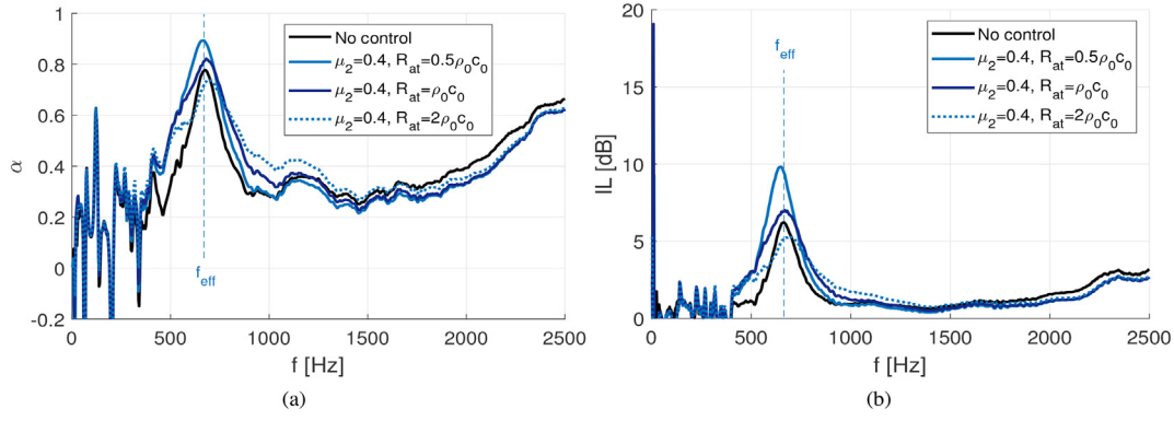
Fig. 8. Effect of the variation of the target resistance ( R_{at} = [0.5\rho_0c_0, \rho_0c_0, 2\rho_0c_0] ) and control law parameters ( \mu_1 = \mu_2 = 0.4 ): a) Absorption coefficient ( \alpha ), b) Insertion loss (IL).
