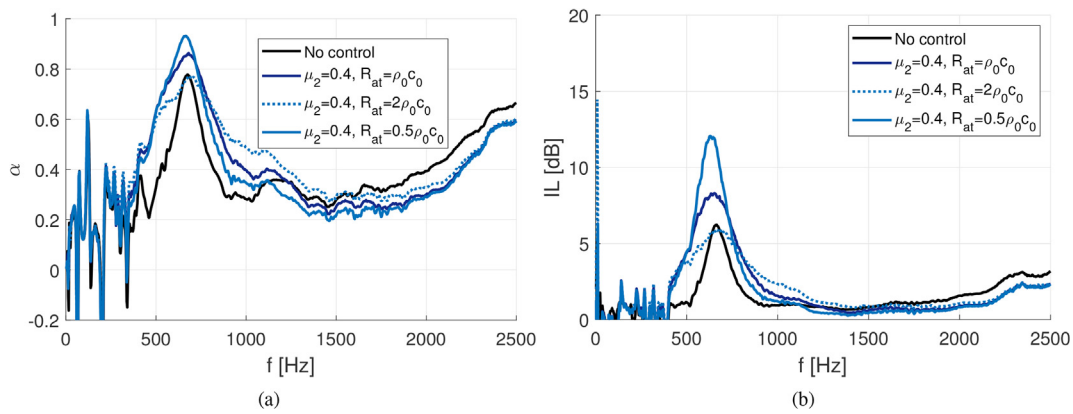
Fig. 11. Effect of the variation of the target resistance ( R_{at} = [\rho_0 c_0, 2\rho_0 c_0, 0.5\rho_0 c_0] ) and control law parameters ( \mu_1 = \mu_2 = 0.4 ). Transport speed of the advection condition ( H_{nonloc} : c_a = 0.9c_0 ): a) Absorption coefficient ( \alpha ), b) Insertion loss (IL).
