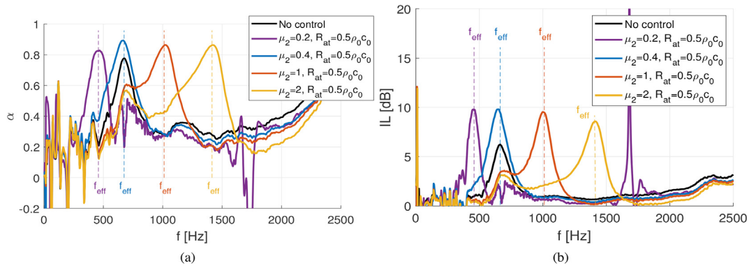
Fig. 9. Effect of the variation of the parameters of the control law ( \mu_1 = 0.4, \mu_2 = [0.2, 0.4, 1, 2] ) and target resistance ( R_{at} = 0.5\rho_0c_0 ): a) Absorption coefficient ( \alpha ), b) Insertion loss (IL).
