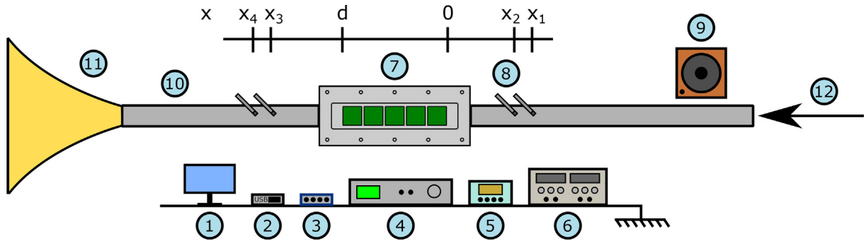
Fig. 4. Experimental setup diagram of the Caïman wind tunnel tests.
