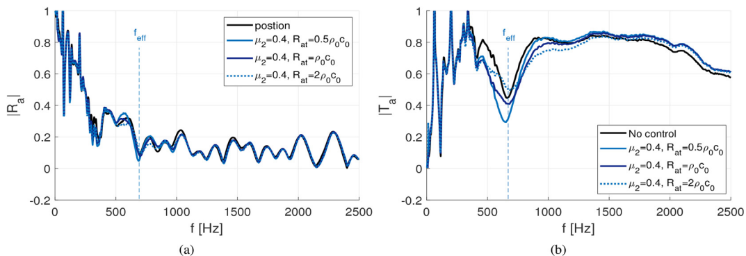
Fig. 7. Effect of the variation of the target resistance ( R_{\text{at}} = [0.5\rho_0 c_0, \rho_0 c_0, 2\rho_0 c_0] ) and control law parameters ( \mu_1 = \mu_2 = 0.4 ): a) Reflexion coefficient ( |R_a| ), b) Transmission coefficient ( |T_a| ).
