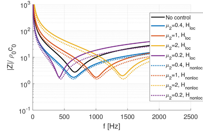
Fig. 18. Effective impedance in the treated surface for experimental results.
