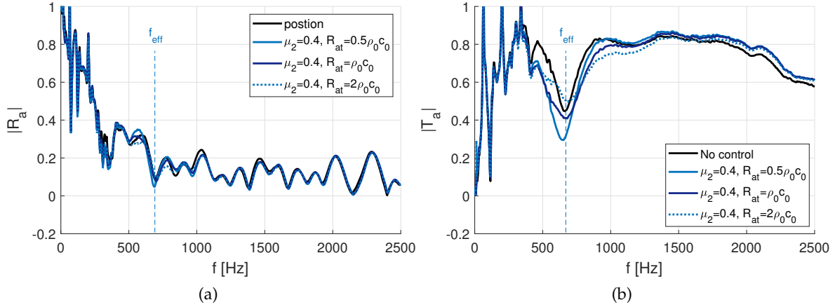
FIGURE 7. Effect of the variation of the target resistance ( R_{at} = [0.5\rho_0c_0, \rho_0c_0, 2\rho_0c_0] ) and control law parameters ( \mu_1 = \mu_2 = 0.4 ): a) Reflexion coefficient ( |R_a| ), b) Transmission coefficient ( |T_a| ).
