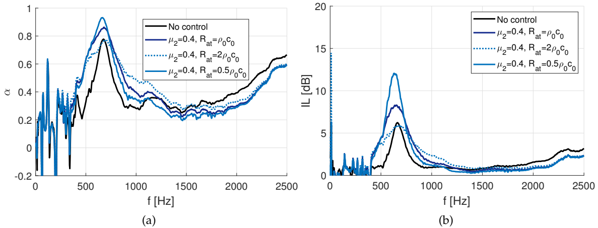
FIGURE 11. Effect of the variation of the target resistance ( R_{at} = [\rho_0c_0, 2\rho_0c_0, 0.5\rho_0c_0] ) and control law parameters ( \mu_1 = \mu_2 = 0.4 ). Transport speed of the advection condition ( H_{nonloc} : c_a = 0.9c_0 ): a) Absorption coefficient ( \alpha ), b) Insertion loss (IL).
