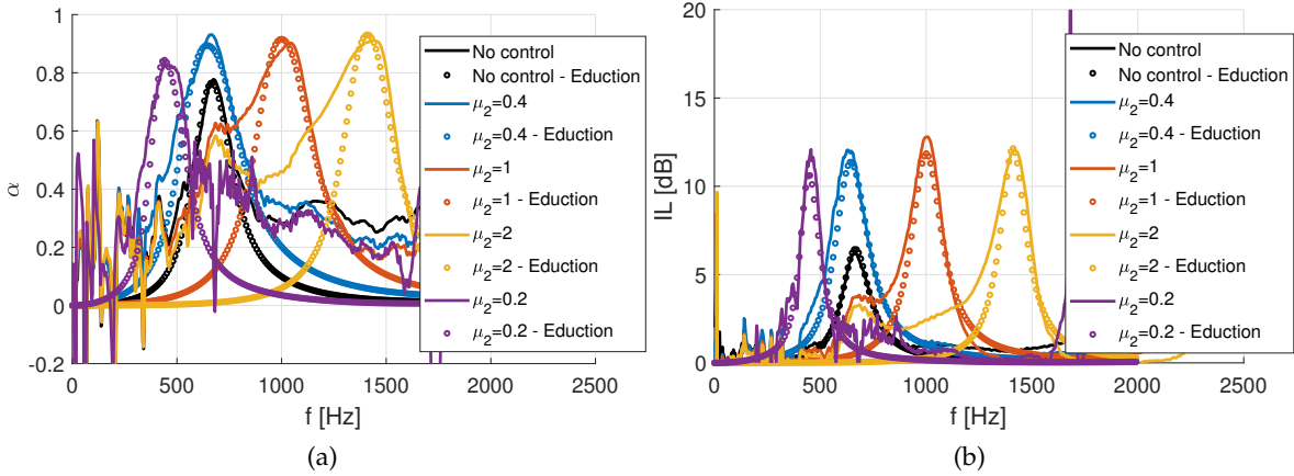
FIGURE 17. Eduction - Variation of the parameters of the control law ( \mu_1 = 0.4 , \mu_2 = [0.2, 0.4, 1, 2] ), Transport speed of the advection condition ( H_{nonloc} : c_a = 0.9c_0 ), Target resistance ( R_{at} = 0.5\rho_0c_0 ): a) Absorption coefficient ( \alpha ), b) Insertion loss (IL).
