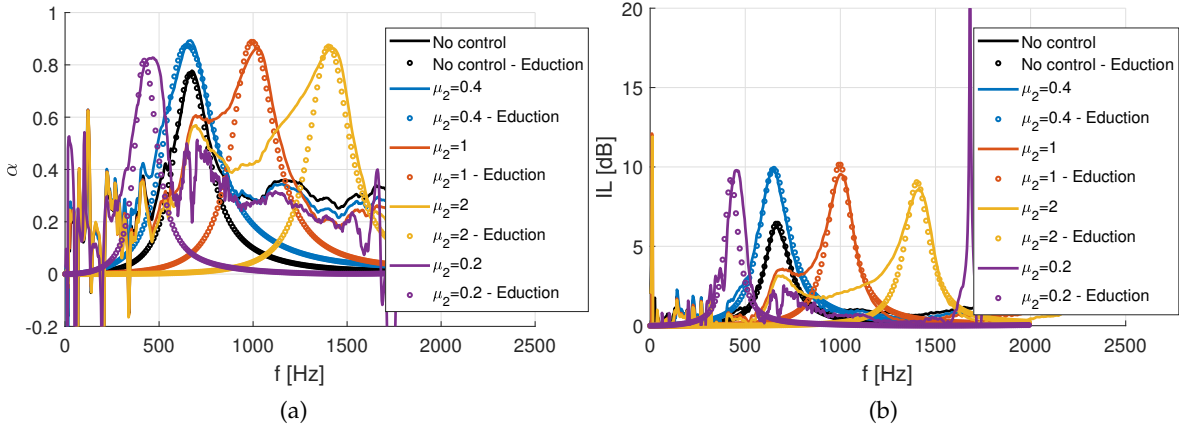
FIGURE 16. Eduction - Variation of the parameters of the control law ( \mu_1 = 0.4 , \mu_2 = [0.2, 0.4, 1, 2] ), Target resistance ( R_{at} = 0.5\rho_0c_0 ): a) Absorption coefficient ( \alpha ), b) Insertion loss (IL).
