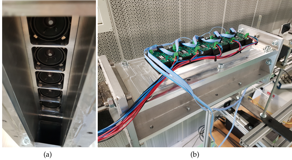
FIGURE 6. Active cells mounted in the Caiiman wind tunnel : a) inside view (without wiremesh), b) outside view.
