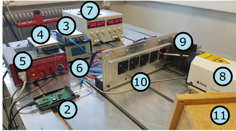
FIGURE 3. Experimental setup picture of the microphones calibration and Thiele-Small cell parameters identification.
