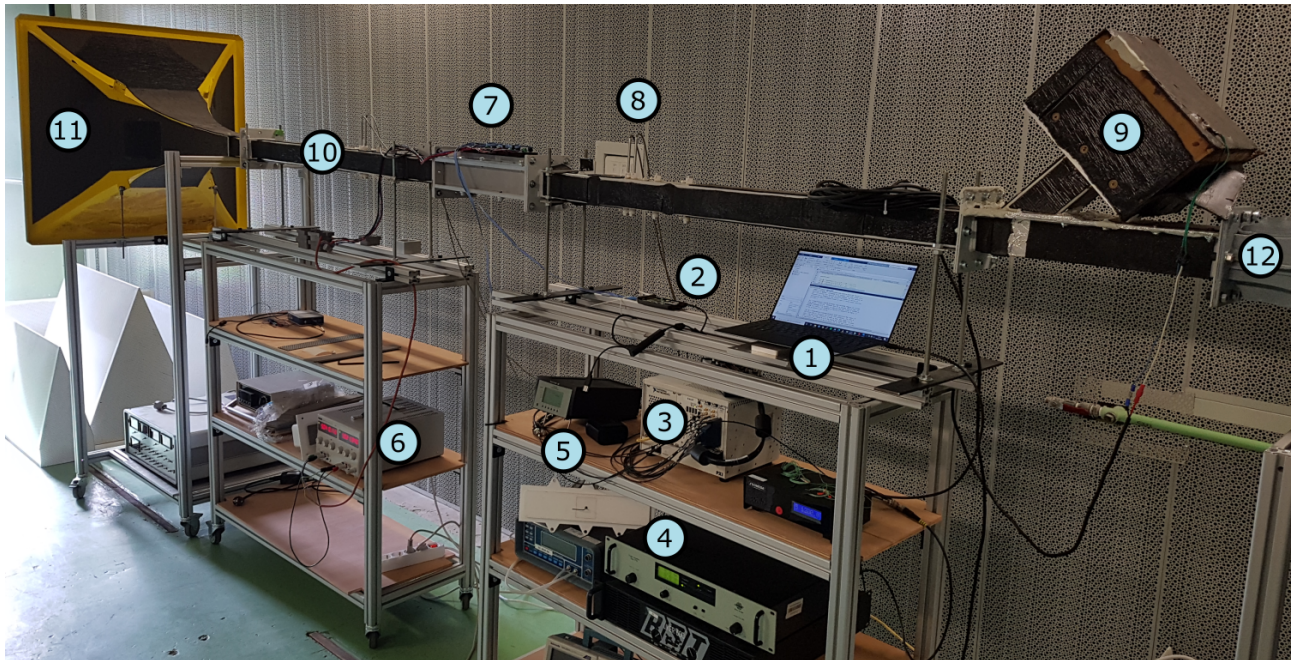
FIGURE 5. Experimental setup picture of the Caïman wind tunnel tests.
