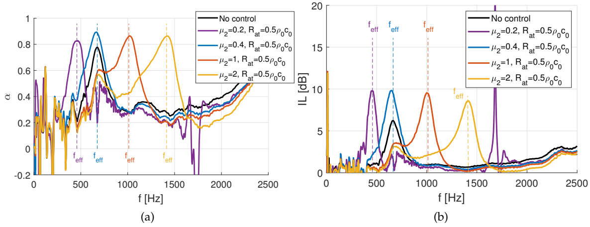
FIGURE 9. Effect of the variation of the parameters of the control law ( \mu_1 = 0.4 , \mu_2 = [0.2, 0.4, 1, 2] ) and target resistance ( R_{at} = 0.5\rho_0c_0 ): a) Absorption coefficient ( \alpha ), b) Insertion loss (IL).
