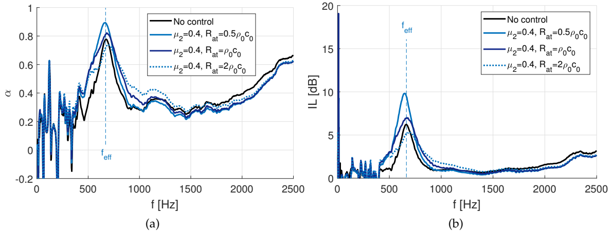
FIGURE 8. Effect of the variation of the target resistance ( R_{at} = [0.5\rho_0c_0, \rho_0c_0, 2\rho_0c_0] ) and control law parameters ( \mu_1 = \mu_2 = 0.4 ): a) Absorption coefficient ( \alpha ), b) Insertion loss (IL).
