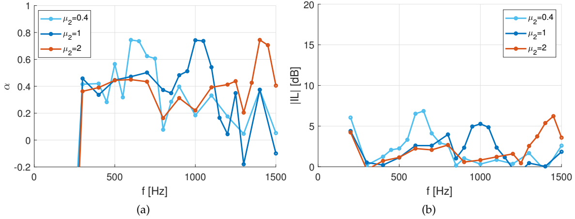
FIGURE 13. Effect of the variation of the parameters of the control law ( \mu_1 = 0.4 , \mu_2 = [0.4, 1, 2] ) and flow velocity (100 m/s) : a) Absorption coefficient ( \alpha ), b) Insertion loss (IL).
