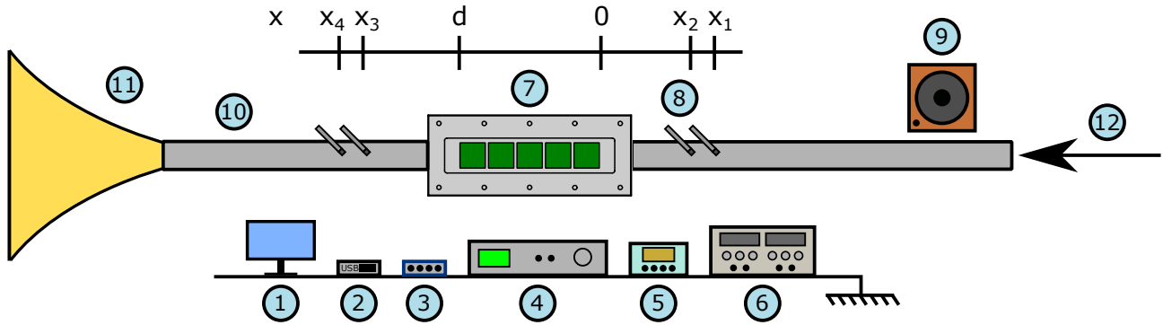
FIGURE 4. Experimental setup diagram of the Caïman wind tunnel tests.
