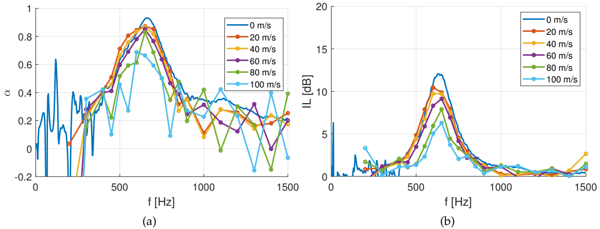
FIGURE 14. Effect of the variation of flow velocity [20, 40, 60, 80, 100] m/s and control law parameters ( \mu_1 = \mu_2 = 0.4 ). Transport speed of the advection condition ( H_{nonloc} : c_a = 0.9c_0 ) : a) Absorption coefficient ( \alpha ), b) Insertion loss (IL).
