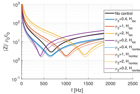
FIGURE 18. Effective impedance in the treated surface for experimental results.
