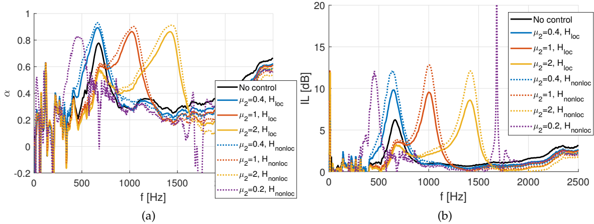
FIGURE 10. Effect of the variation of the parameters of the control law ( \mu_1 = 0.4, \mu_2 = [0.2, 0.4, 1, 2] ) and target resistance ( R_{at} = 0.5\rho_0c_0 ). Transport speed of the advection condition ( H_{nonloc} : c_a = 0.9c_0 ): a) Absorption coefficient ( \alpha ), b) Insertion loss (IL).
