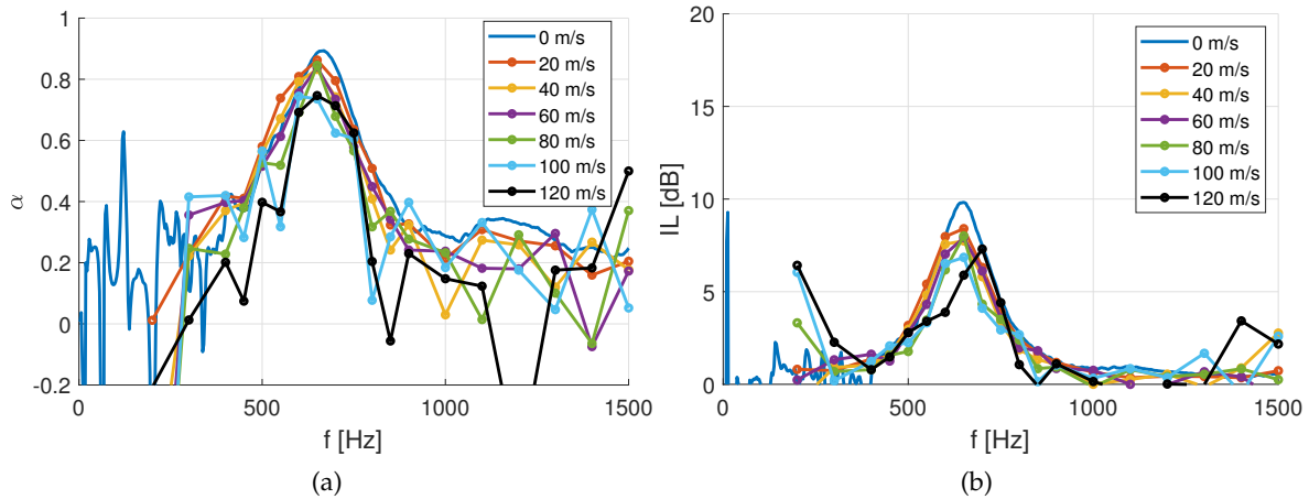
FIGURE 12. Effect of the variation of flow velocity [20, 40, 60, 80, 100, 120] m/s and control law parameters ( \mu_1 = \mu_2 = 0.4 ): a) Absorption coefficient ( \alpha ), b) Insertion loss (IL).
