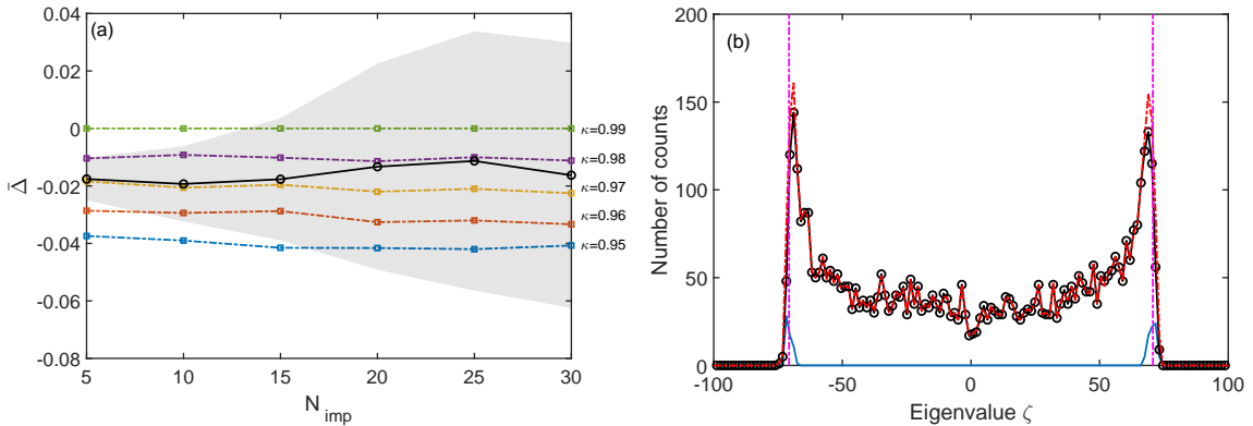
Figure 7: (color online) a) The relative difference between the average number of detected and imprinted solitons \bar{\Delta} (black open markers with solid black line) with average uncertainty represented by the gray shaded area as a function of the number of imprinted solitons N_{\text{imp}} . The different dashed-dotted lines with square markers represent the value of \Delta as a function of N_{\text{imp}} with phases below a certain value, |\phi| < \kappa\pi/2 . Here we only plot five different \kappa values ranging from \kappa = 0.95 to \kappa = 0.99 . b) Histogram of soliton eigenvalues, computed for a state with 10 imprinted solitons N_{\text{imp}} = 10 , averaged over 500 realizations. The black solid line with open circles shows the histogram computed for eigenvalues identified by the threshold \epsilon_- , the blue solid line shows the histogram for extra eigenvalues identified only by the threshold \epsilon_+ and the dashed-dotted red line the expected distribution of imprinted solitons. The dash-dotted vertical magenta lines correspond to \pm c/2 .
