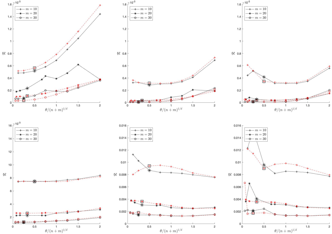
Figure 6: MSE of \widehat{\text{ISE}} for \zeta^{\text{BQ}^*} (black) and \zeta_K^{\text{BQ}} (red) for m \in \{10, 20, 30\} . From left to right \nu = 1/2, 3/2, 5/2 . Statistics over 500 realisations. Top: Q is the Matérn 3/2 kernel, bottom: Q is the Cauchy kernel; d = 1 .
