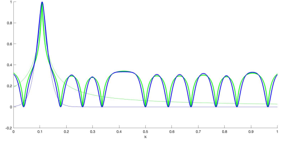
Figure 2: \overline{K}|_n(\mathbf{z}_1, \mathbf{x})/\overline{K}|_n(\mathbf{z}_1, \mathbf{z}_1) (bold lines) and K(\mathbf{z}_1, \mathbf{x})/K(\mathbf{z}_1, \mathbf{z}_1) (thin lines) for the Cauchy and Matérn kernels used in Figure 1 (same colour code) and z_1 \simeq 0.1 .
