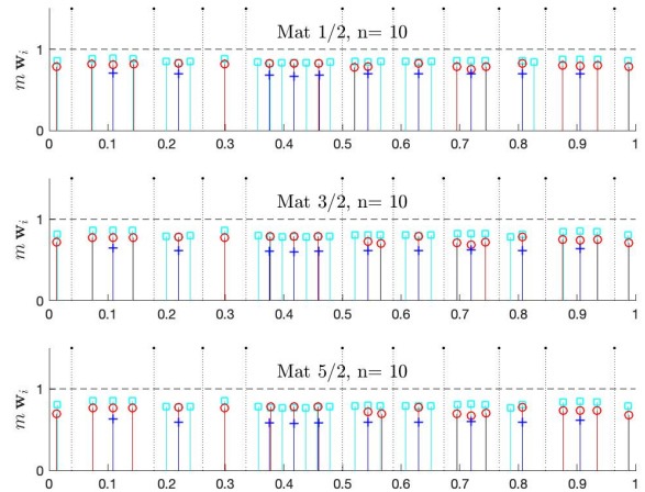
Figure 14: \zeta^{\text{BQ}^*} in Figure 11, \theta = 2(n+m)^{1/d} .
