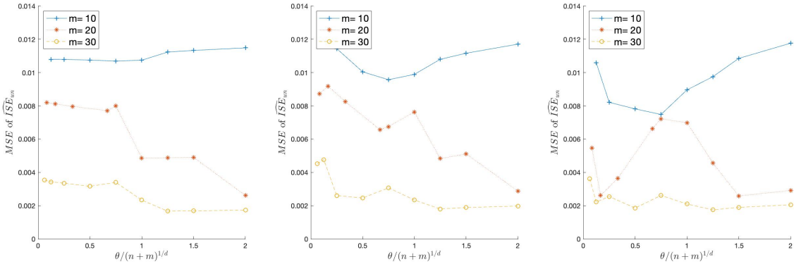
Figure 5: MSE of \widehat{ISE}_{u,n} . Statistics over 500 realisations for the example in Figure 3
