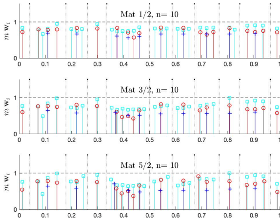
Figure 13: \zeta^{\text{BQ}^*} in Figure 11, \theta = (n+m)^{1/d} .
