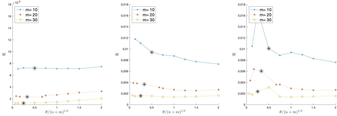
Figure 4: MSE of \widehat{ISE} . Statistics over 500 realisations. Q is a Cauchy kernel, K is as in Figure 3; d = 1 .
