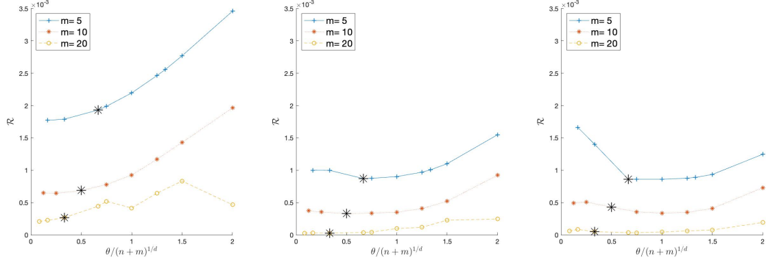
Figure 3: MSE of \widehat{ISE} . Statistics over 500 realisations. Q is a Matérn 3/2 kernel; K is a Matérn kernel with \nu = 1/2 (left), \nu = 3/2 (middle) and \nu = 5/2 (right); d = 1 .
