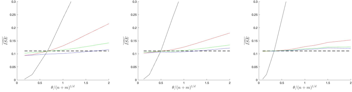
Figure 16: \text{IMSE}^*(\mathbf{X}_n; \theta) (black), \overline{\text{ISE}} (dashed), \overline{\text{ISE}}_{\text{biased}}(\theta) (blue), \overline{\text{ISE}}_{\text{affine}}(\theta) (red) and \overline{\text{ISE}}_{\text{linear}}(\theta) (green). From left to right m = 5, 10, 20 . Q and K are the Matérn 3/2 kernel.
