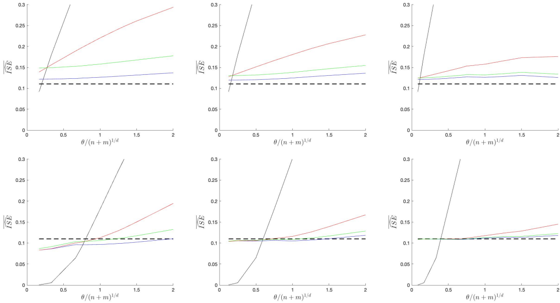
Figure 17: \text{IMSE}^*(\mathbf{X}_n; \theta) (black), \overline{\text{ISE}} (dashed), \overline{\text{ISE}}_{\text{biased}}(\theta) (blue), \overline{\text{ISE}}_{\text{affine}}(\theta) (red), \overline{\text{ISE}}_{\text{linear}}(\theta) (green). From left to right m = 5, 10, 20 . Q is the Matérn 3/2 kernel; K is the Matérn kernel with parameter \nu = 1/2 (top) and \nu = 5/2 (bottom).
