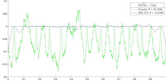
Figure 15: Bias of \hat{\varepsilon}^2 , \mathbf{x} \in \mathcal{X} . (simulations from Cauchy and Matérn 3/2 kernels).
