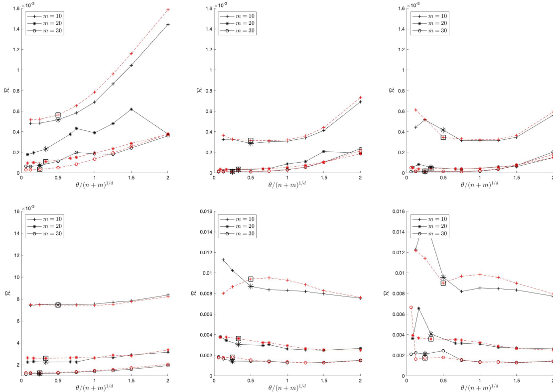
Figure 6: MSE of \widehat{\text{ISE}} for \zeta^{\text{BQ}*} (black) and \zeta^{\text{BQ}} (red) for m \in \{10, 20, 30\} . From left to right \nu = 1/2, 3/2, 5/2 . Statistics over 500 realisations. Top: Q is the Matérn 3/2 kernel, bottom: Q is the Cauchy kernel; d = 1 .
