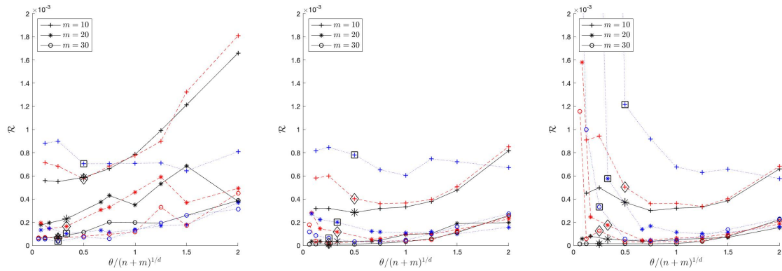
Figure 8: MSE of \widehat{ISE} for \zeta^{BQ*} (black solid lines), \zeta_K^{KH} (red dashed lines) and \zeta^{KH*} (dotted blue lines), for m = 10 (+), m = 20 (*) and m = 30 (o). From left to right \nu = 1/2, 3/2, 5/2 . Q is a Matérn 3/2 kernel; d = 1 .
