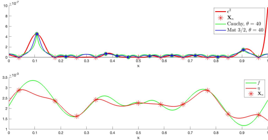
Figure 1: Top: \varepsilon^2(\mathbf{x}) (red) and \widehat{\varepsilon}^2_{\mathcal{F}_n}(\mathbf{x}|\mathbf{Z}_m) (blue and green) for two distinct GP models. Down: f , \eta and \mathbf{X}_n .
