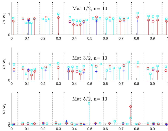
Figure 12: \zeta^{\text{BQ}^*} in Figure 11, \theta = n^{1/d} .
