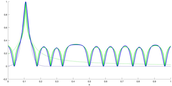
Figure 2: \overline{K}_{|n}(\mathbf{z}_1, \mathbf{x})/\overline{K}_{|n}(\mathbf{z}_1, \mathbf{z}_1) (bold lines) and K(\mathbf{z}_1, \mathbf{x})/K(\mathbf{z}_1, \mathbf{z}_1) (thin lines) for the Cauchy and Matérn kernels used in Figure 1 (same colour code) and z_1 \simeq 0.1 .
