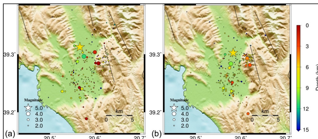
Figure 3. Relief map showing locations of epicentres (solid circles) of the 2020 Kanallaki earthquake sequence (a) before and (b) after relocation with HypoDD. Colours correspond to the focal depths. The star represents the epicentre of the M_w = 5.6 mainshock of 21 March 2020.
