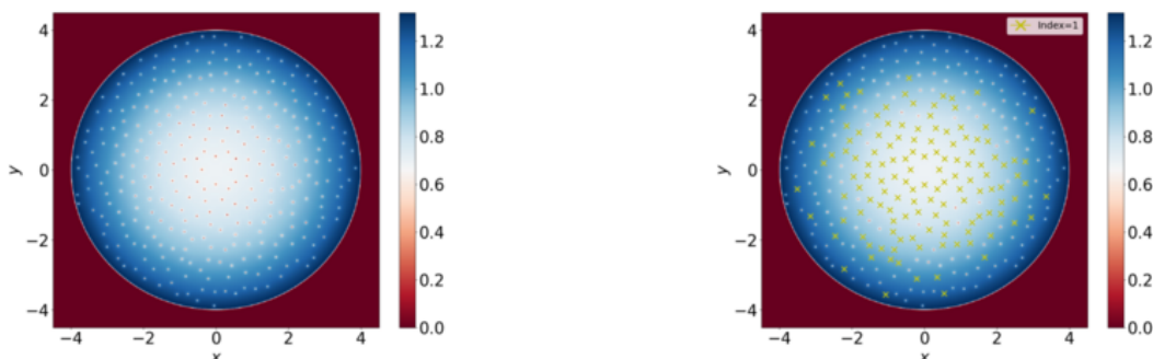
FIGURE 7. The squared modulus of a minimizer for \Omega = 20 , \varepsilon = 10^{-2} . In the right panel, the numerical computation of the indices of the vortices is carried out with N_{min} = 1 , N_{max} = 3 , tol_1 = 0.1 and tol_2 = 0.05 .
