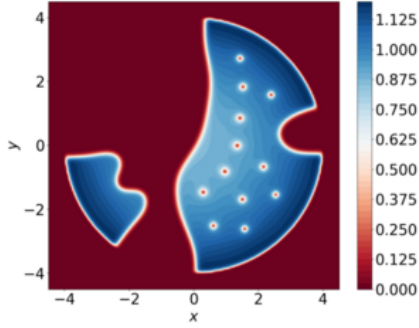
(A) First component of a minimizer of the energy E_\epsilon^\Delta using the EPG method.
