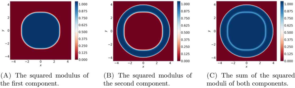
FIGURE 12. The squared modulus of the first component (A) and of the second component (B) for a minimizer in the case of two components condensate with no rotation and \delta = 1.5 . Their sum is displayed in Fig. (C).
