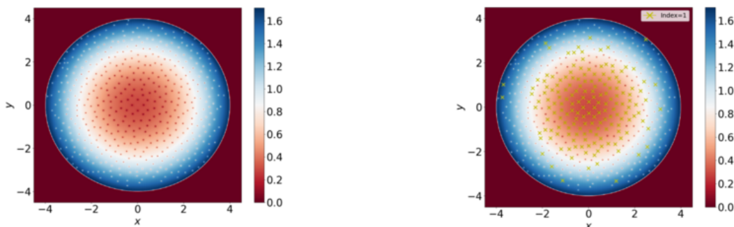
FIGURE 8. The squared modulus of a minimizer for \Omega = 30 , \varepsilon = 10^{-2} . In the right panel, the numerical computation of the indices of the vortices is carried out with N_{min} = 1 , N_{max} = 3 , tol_1 = 0.05 and tol_2 = 0.02 .
