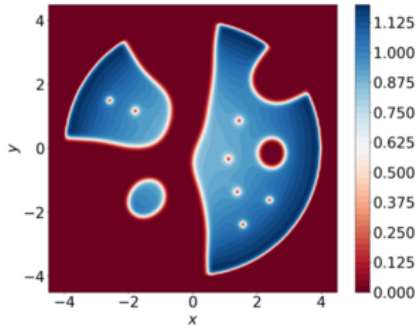
(C) First component of a minimizer of the energy E_\epsilon^\Delta using the GPELab method.
