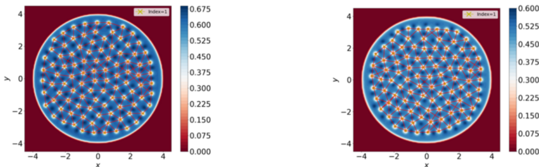
(A) The vortices indexes of the first component.
