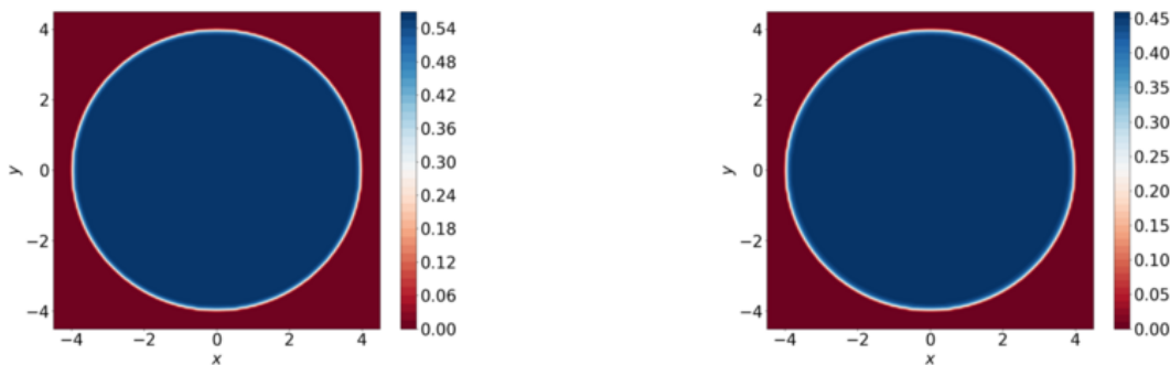
(A) The squared modulus of the first component.
