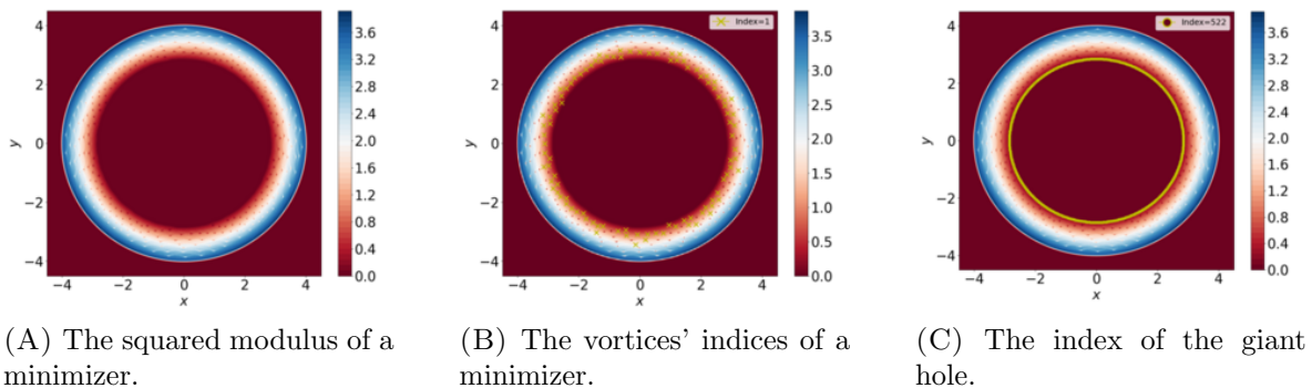
FIGURE 10. The squared modulus (A) of a minimizer of the energy for \Omega = 70 , \varepsilon = 10^{-2} . The vortices' indices of a minimizer of the energy (B) detected with N_{min} = 1 , N_{max} = 3 , tol_1 = 0.05 and tol_2 = 0.02 . The index of the giant hole (C) detected with r = 2.85 (see Remark 5).
