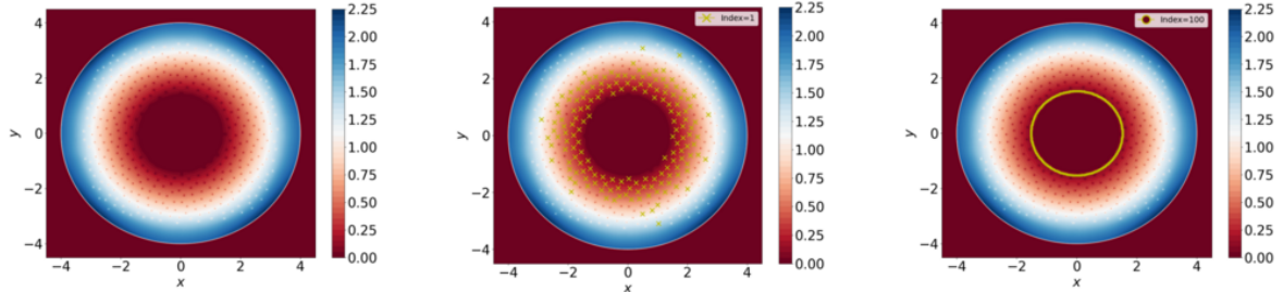
(A) The squared modulus of a minimizer.
