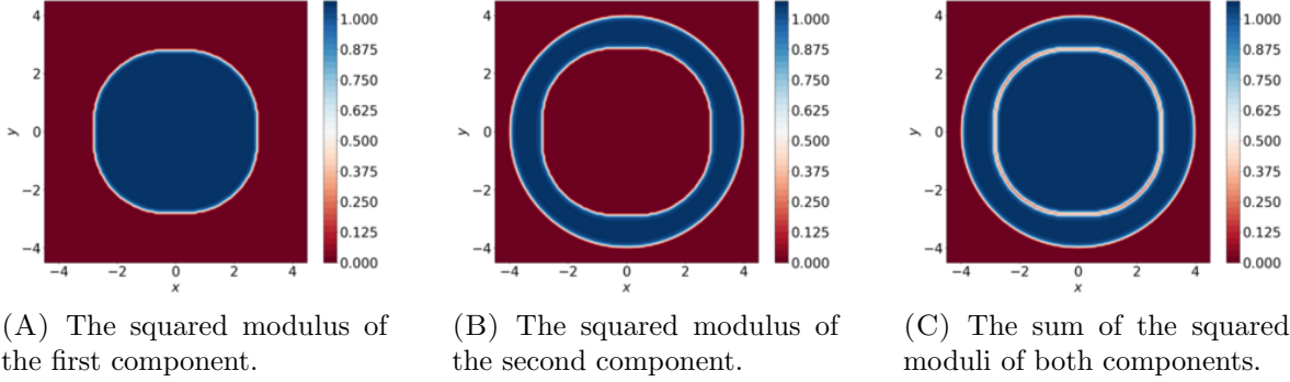
FIGURE 11. The squared modulus of the first component (A) and the second component (B) for a minimizer in the case of two components condensate with no rotation and \delta_\varepsilon = 4000 . Fig (C) displays their sum.
