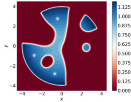
(D) Second component of a minimizer of the energy E_\epsilon^\Delta using the GPELab method.
