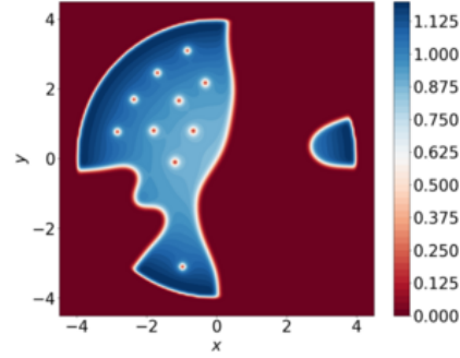
(B) Second component of a minimizer of the energy E_\epsilon^\Delta using the EPG method.
