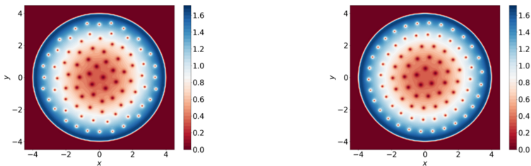
(A) A minimizer of the energy E_\varepsilon^\Delta using the EPG method.
