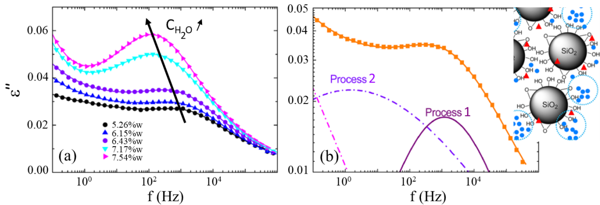
Fig. 10. Dielectric loss spectra of hydrated silica NPs at T = 146 K. The solid lines through the data points represent fits to the experimental data using the sum of two Cole-Cole functions ( \delta = 1 in Eq. (3)) and a conductivity term. a NPs at different water concentrations, b decomposition of the dielectric response of NPs containing 6.4%w of water. At this temperature, processes 1 (solid line, water) and 2 (dashed-dotted line, silanols) are observed. Note that they are termed processes 2 and 3, respectively, in the original publication [39]. Inset: schematic drawing of the water adsorbed at the silica surface (blue dots: hydrogen bond water, red triangles irrotational water). Water molecules are distributed homogeneously or grouped to form clusters at high concentration (dotted circles). Adapted from [39].
