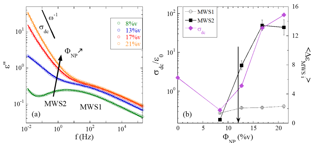
Fig. 13. a Dielectric loss spectra at 333 K for 50%F-SB PNCs with different \Phi_{NP} . Solid lines are fits by the sum of two HN functions and a dc-conductivity term. b DC-conductivity at 393 K (diamonds) and average value of the dielectric strengths over T for MWS1 (circles) and MWS2 (squares) as a function of filler fraction for the same PNCs. The percolation threshold as obtained from rheology is indicated by an arrow. Adapted from [42].
