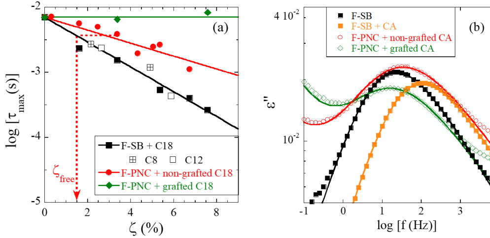
Fig. 19. a BDS segmental relaxation time at T = 258 K as a function of the nominal silane matrix concentration \zeta in F-SB. Calibration curve for polymer with various amounts of silane, C 8 (crossed empty squares), C 12 (empty squares) and C 18 (plain squares), in F-SB. The solid black line represents a linear fit to all silanes in log-representation. The data for PNCs without (resp. with) activation of the grafting reaction are superimposed (red circles, resp. green diamonds) for nominal \zeta in samples, together with a linear fit for the non-grafted PNCs. The construction (red dotted lines) illustrates the determination of the effective \zeta_{\text{free}} within the matrix in presence of NPs. b Dielectric loss spectra at T = 258 K of F-SB (without and with C 18 at \zeta = 3.4\% ) and F-PNCs ( \Phi_{\text{NP}} \approx 10\% v, same amount of C 18 ). Possible silane grafting is indicated in the legend. Solid lines represent the fit to the experimental data based on Eq. (3) plus a purely dissipative dc-conductivity term. Adapted from [80].
