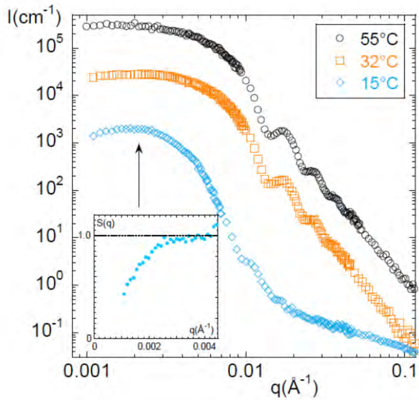
Figure 1.6: Structure of pNNPAM microgel in D_2O for three different temperatures as indicated in the legend. The SANS intensities at 32^\circ C and 55^\circ C have been vertically shifted by a factor of 10 (resp. 100). In the inset, an estimate of the structure factor is shown for the lowest temperature.
