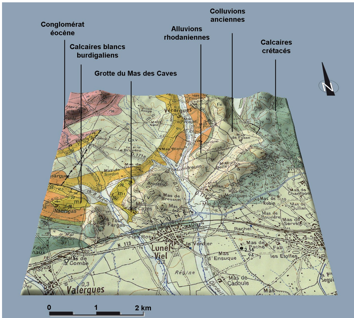
Fig. 1 - Geographical location of the caves of Mas des Caves (courtesy L. Bruxelles). Calcaires Crétaçés: Cretaceous limestone; colluvions anciennes: old colluviums; alluvions Rhodaniennes: Rhodanian alluviums (quartz, quartzite, flint, metamorphic, limestone); calcaires blanc Burdigaliens: white Burdigalian limestone; conglomérat Eocène: Eocene conglomerate.
