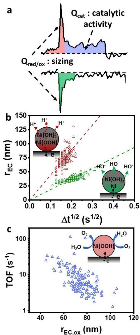
Figure 4: (a) Analysis of an individual current signal for oxidative and reductive nanoimpacts. (b) NP radius vs the square root of peak duration for E_{\text{C UME}} = -0.6 V (green) and +1 V (red). Dotted lines: linear fits to determine the diffusion coefficients of \text{HO}^- (green) and \text{H}^+ (red) within the NPs using Equation (8). (c) Turnover frequency (TOF) of individual NPs as a function of their electrochemical radius r_{\text{EC,ox}} .
