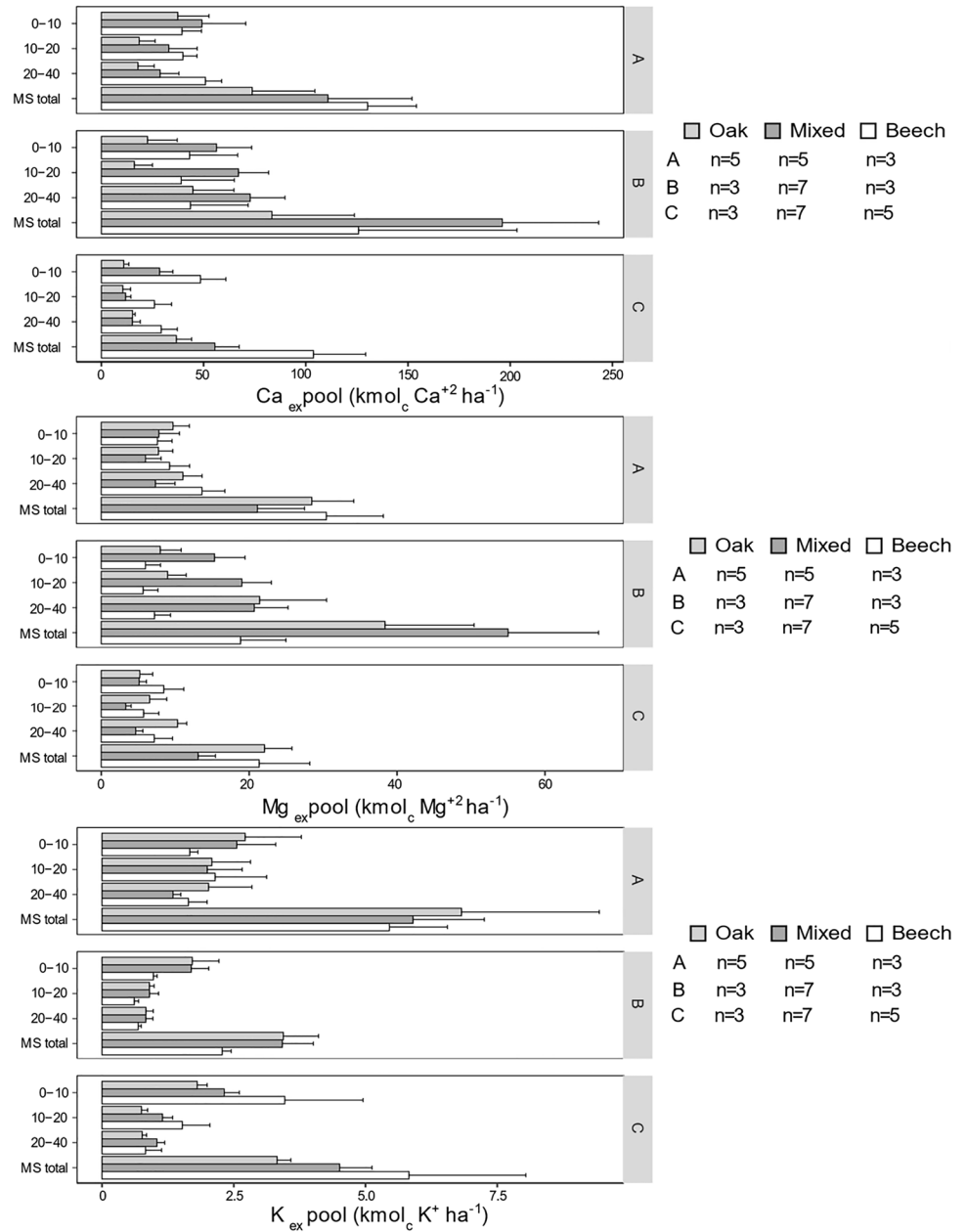
Fig. 9 Means (and SE) of the pool of BaCl 2 -exchangeable basic cations in the mineral soil of the beech, mixed (beech-oak) and oak stands of the three transects A–C ( n =number of plots). Profile totals (MS total) for Ca +2 ex , Mg +2 ex and K + ex are given for a depth of –40 cm. No samples were taken in the linden forests
