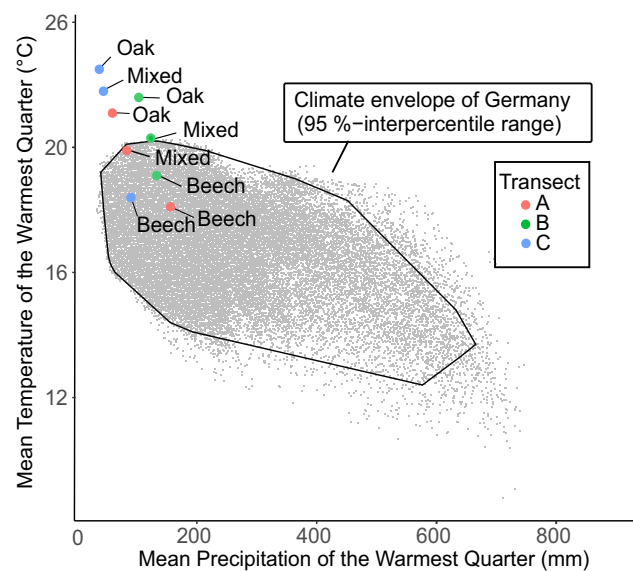
Fig. 2 Location of the oak, mixed forest and beech plots of the three transects (red: transect A, green: transect B, blue: transect C) in a biplot of mean temperature of the warmest quarter (BIO10) and mean precipitation of the warmest quarter (BIO18), relative to the climate stations of Germany (grey dots). The black line encloses the 95% inter-percentile range of German climate stations, which is used as a rough approximation of the climate envelope of beech in Central Europe. The climate data were extracted from the CHELSA climate data base (Karger et al., 2017)
