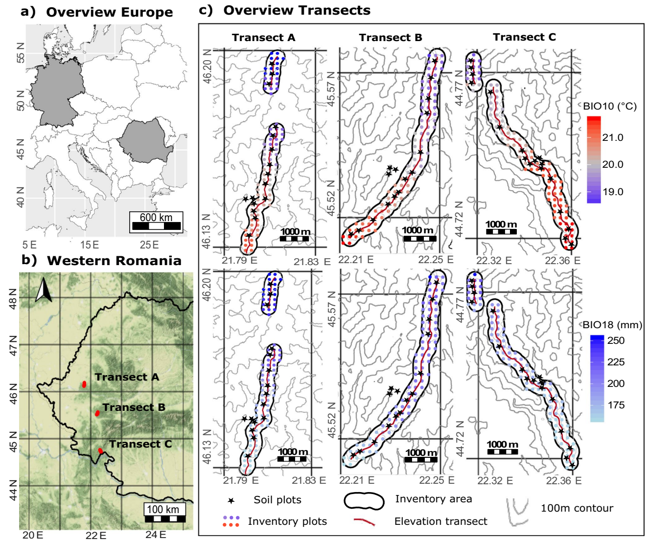
Fig. 1 a Location of Romania in Europe, b location of the three transects A–C in western Romania from the R package rworldmap (South, 2011) and c maps of the three transects with coordinates, contour lines (100-m elevation distance), the inventoried forest area and location of inventory and soil sampling plots. The colour of the dots
