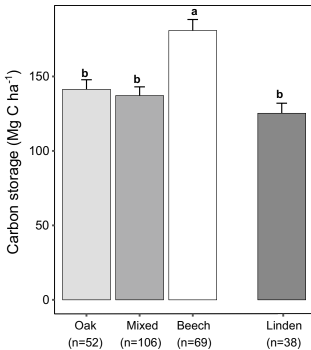
Fig. 3 Store of aboveground biomass carbon (in Mg C ha -1 ) in the oak, mixed and beech forest plots (means and standard error (SE) of the three transects). Plots dominated by linden (basal area of T. tomentosa > 66.6%) are also shown. Beech forests: all plots with basal area of F. sylvatica > 66.6%, oak forests: all plots with basal area of Quercus species > 66.6%, mixed forests: all other forests (except for stands with T. tomentosa > 66.6%). Significant differences between forest types ( p \leq 0.05 ) are marked with different small letters (one-way ANOVA with post hoc Tukey test)
