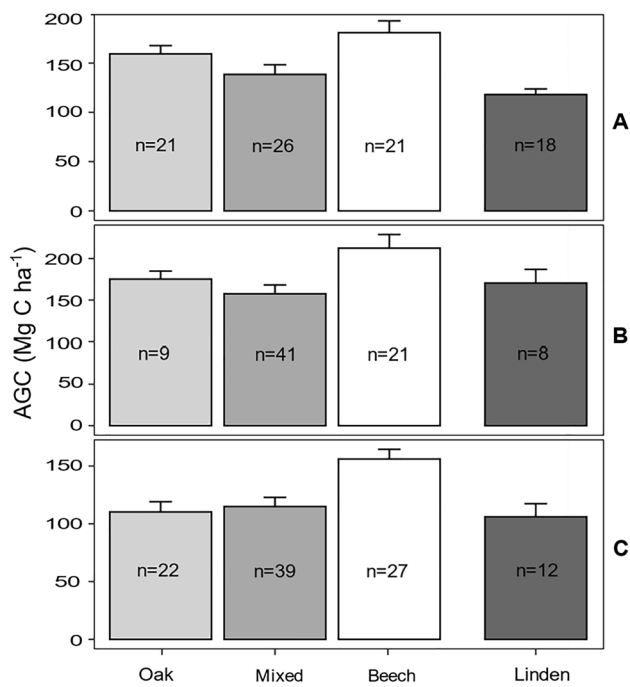
Fig. 7 Store of aboveground carbon (AGC; in Mg C ha -1 ) in the oak, mixed and beech forest plots (means and SE) of each transect A–C. Plots dominated by linden (basal area of T. tomentosa > 66.6%) are also shown. Beech forests: all plots with basal area of F. sylvatica > 66.6%, oak forests: all plots with basal area of Quercus species > 66.6%, mixed forests: all other forests (except for stands with T. tomentosa > 66.6%)
