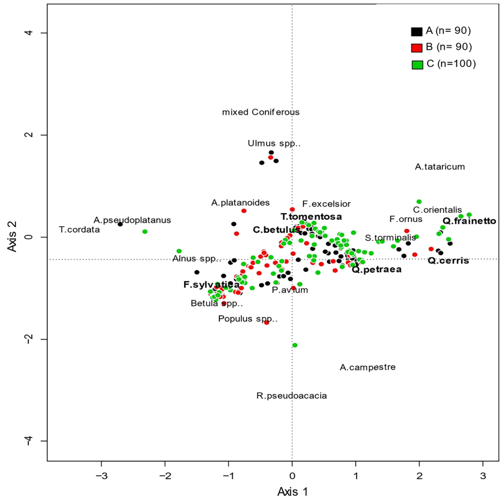
Fig. 10 Detrended correspondence analysis ordination (DCA) calculated with the species' relative basal area, conducted for all species and for the three transects A–C. The plots are marked with different colours for the three transects ( n = number of plots). The main tree species are in bold, minor tree species in normal font
