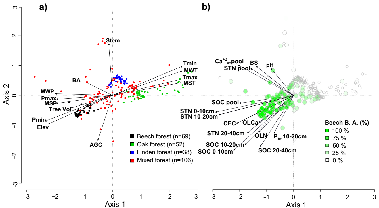
Fig. 5 Climatic, edaphic and stand structural variables significantly ( p < 0.05 ) correlating with the axes 1 and 2 of the DCA ordination space calculated with the tree species' relative basal area (B.A. in %) in the plots. The relationships are indicated by the direction of arrows, the strength of correlation ( R^2 ) by the arrow lengths. Symbol position was slightly adjusted to avoid overplotting. For variable units of climate, forest stand, organic layer and soil, see Table 2 and for full names with explanations Table 11 in Appendix. Plot (a)
