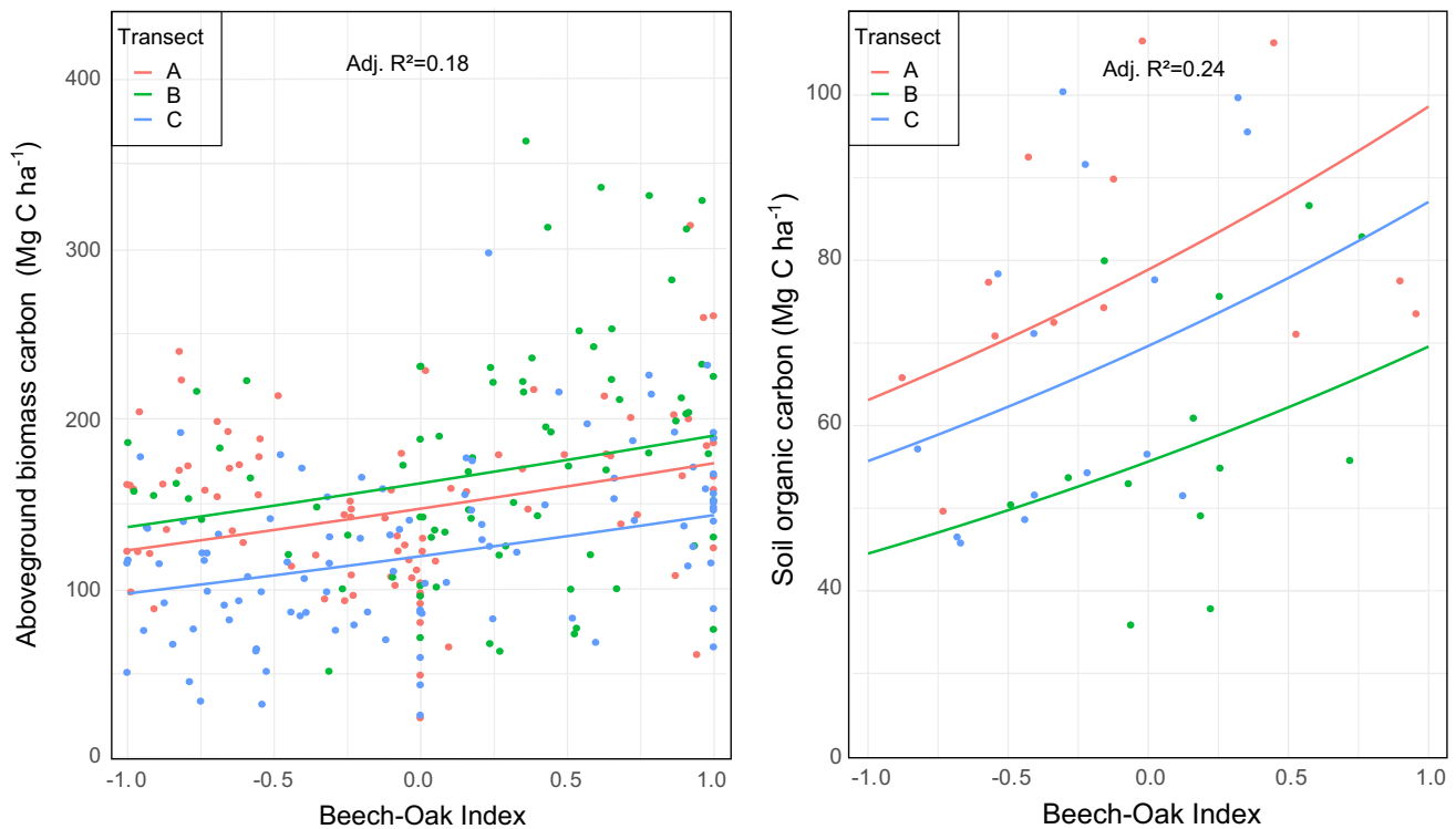
Fig. 6 Left panel: aboveground carbon (Mg C ha -1 ) and right panel: soil organic carbon (Mg C ha -1 ) in dependence of the beech-oak index (-1 for 100% oak to 1 for 100% Beech relative basal area) for the three transects according to the model predictions. The adjusted
