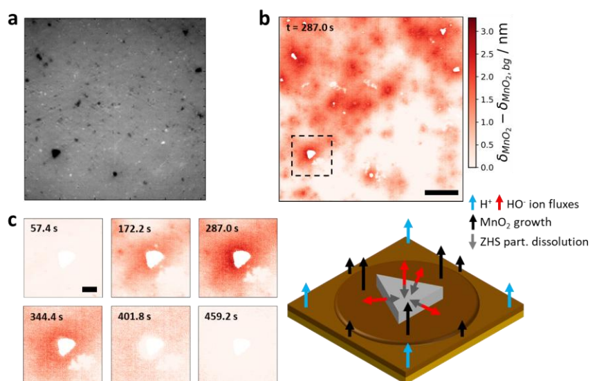
Figure 6. Operando imaging of the first galvanostatic charge-discharge cycle of a Zn-MnO 2 battery in ZHS-saturated 2 mM MnSO 4 + 2 M ZnSO 4 . a) Background subtracted optical reflectometry image of the Au cathode coated with ZHS particles (dark-contrasted features). b) Reflectivity image converted into relative MnO 2 thickness, \delta_{\text{MnO}_2} - \delta_{\text{MnO}_2, \text{bg}} . The particles detected in a) are masked to highlight that they are surrounded by regions of thicker MnO 2 deposits. Scale bar: 50 \mu\text{m} . c) Sequential relative MnO 2 thickness images showing the expansion of the excess deposition region around a ZHS particle (zoom inside the dashed region of interest in b)) and schematic mechanistic explanation. Scale bar: 10 \mu\text{m} .
