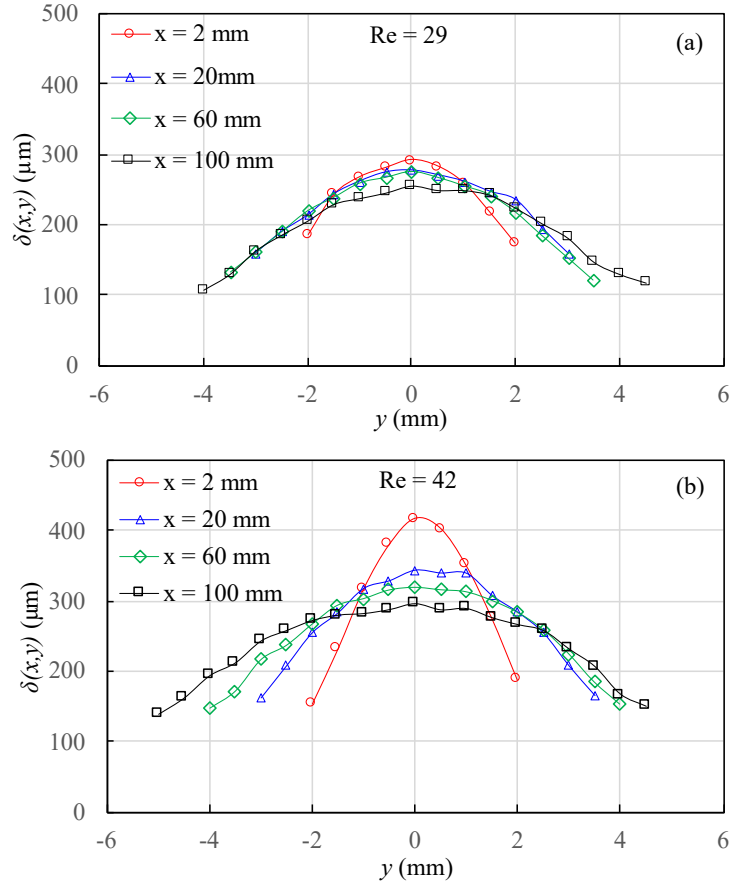
Figure 5. Spanwise rivulet profile at x = 2, 20, 60, 100 \text{ mm} from the bottom edge of the perforation. Plate thickness t = 1 \text{ mm} , perforation diameter d = 4 \text{ mm} . Curtain mode. (a) \text{Re} = 29 ; (b) \text{Re} = 42 . The lines linking the dots are intended to guide the eye along the data points.
