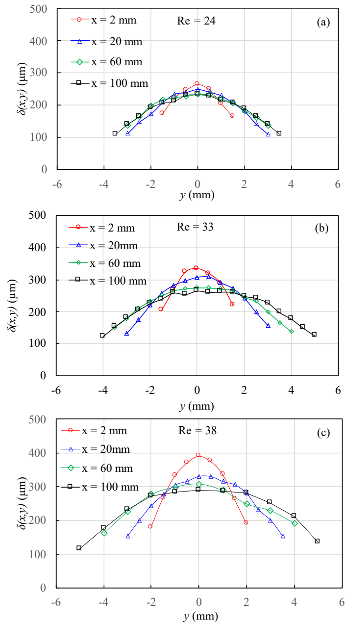
Figure S4. Spanwise rivulet profile at x = 2, 20, 60, 100 mm from the bottom edge of the perforation. Plate thickness t = 1 mm, perforation diameter d = 4 mm. Curtain mode. (a) \text{Re} = 24 ; (b) \text{Re} = 33 = \text{Re}_{cr} ; (c) \text{Re} = 38 . The lines linking the dots are intended to guide the eye along the data points.
