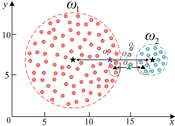
Fig. 3. Illustration of the simulated cluster centers based on imbalanced data.
