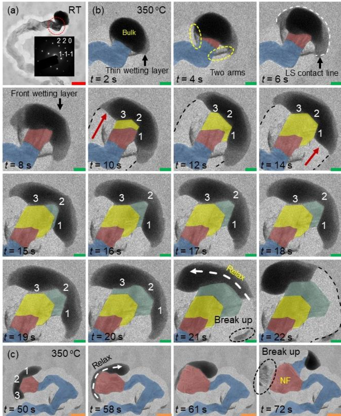
Figure 1. In situ TEM observation of an IPSLS Si NW growth at 350 °C. (a) TEM image taken at room temperature of a Si NW grown on a SiN x membrane at 400 °C. Inset: selected area electron diffraction pattern in [1-12] zone showing the local orientation of c -Si. Two sequences of TEM images extracted from the growth of a NW at 350 °C (Video S1): (b) shows the reactive wetting of a -Si:H coated membrane by a deformed In droplet (from t=2 to 14 s), and the growth of NW in irregular morphology due to the faceted droplet-NW interface
