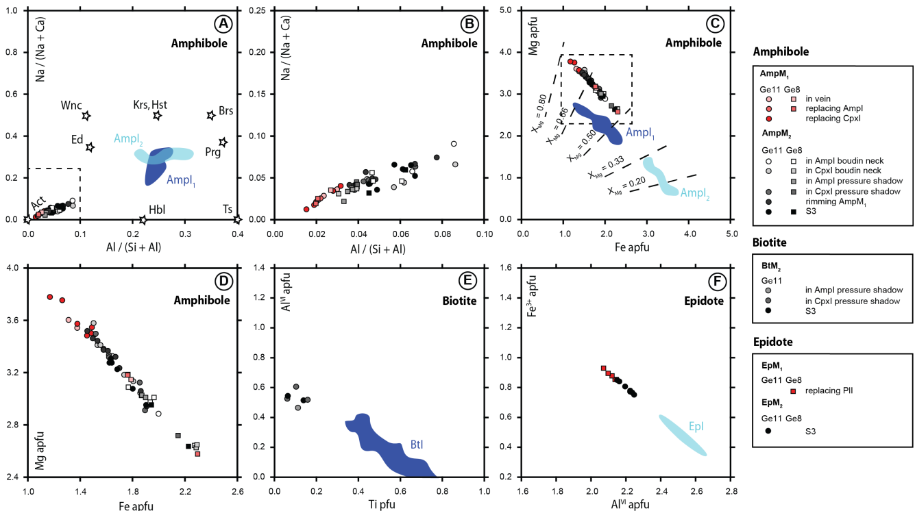
Figure 5. Composition of magmatic (I 1 , I 2 ) and metamorphic (M 1 , M 2 ) minerals in the Edolo diabase. Compositional variations in I 1 and I 2 minerals are reported as blue and light blue shaded areas, respectively. Compositions of M 1 and M 2 minerals are plotted as circles (sample Ge11) and squares (sample Ge8). Red shades highlight different microstructural sites occupied by hydrothermal M 1 minerals. Black shades highlight different microstructural sites occupied by Alpine M 2 minerals. (A): Al/(Al + Si) vs. Na/(Na + Ca) amphibole diagram. Compositional end-members are reported as stars; (B): Enlargement of A. (C): Fe vs. Mg amphibole diagram. X Mg isolines are reported as dashed lines; (D): Enlargement of C; (E): Ti vs. Al VI biotite diagram; (F): Al VI vs. Fe 3+ epidote diagram.
