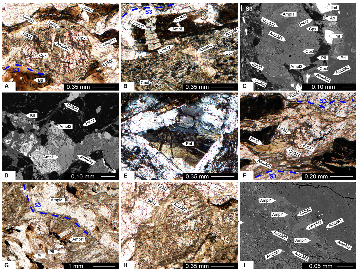
Figure 4. Microstructures of Edolo diabase dykes (plane-polarized light and back-scattered electron images). (A): CpxI and BtI wrapped by S3. S3 is marked by AmpM 2 , BtM 2 , ChlM 2 , and trails of EpM 2 and TtnM 2 . BtI is parallelized to S3. AmpM 2 fills syn-kinematic fractures and pressure shadows around CpxI; (B): CpxI and AmpI are pervasively replaced by ChlM 1 , AmpM 1 , and titanite. Fractures in AmpI and CpxI are syn-kinematic with S3 and filled by AmpM 2 and ChlM 2 ; (C): AmpI, BtI, IlmI, PlI, and CpxI (rimmed by AmpI 2 ) are wrapped by S3 that is marked by AmpM 2 , ChlM 2 , and EpM 2 . Boudin necks are filled by AmpM 2 , PlI is rimmed by PIM 2 ; (D): S3 marked by AmpM 2 , ChlM 2 , and PIM 2 . AmpM 2 fills pressure shadows around zoned AmpI; (E): Interstitial EpI between PlI laths; (F): Relics of EpM 1 within S3 marked by AmpM 2 , BtM 2 , ChlM 2 , EpM 2 , and stylolitic films of TtnM 2 ; (G): Relics of magmatic minerals and AmpM 1 -rich layers within inflected S3; (H): Relic of CpxI wrapped by S3 supported by AmpM 2 , BtM 2 , EpM 2 and minor ChlM 2 ; (I): Micro-boudins of AmpI aligned in S3 foliation: boudin necks are filled by AmpM 2 and ChlM 2 . In the AmpM 1 -rich layer to the right, dark gray cores of AmpM 1 (Al- and Fe-poor) are rimmed by light gray AmpM 2 (Al- and Fe-rich), which marks S3.
