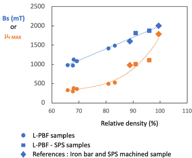
Fig. 10 – Saturation magnetic flux density B_s and maximal relative permeability \mu_{r\ MAX} versus the relative density of the samples.
