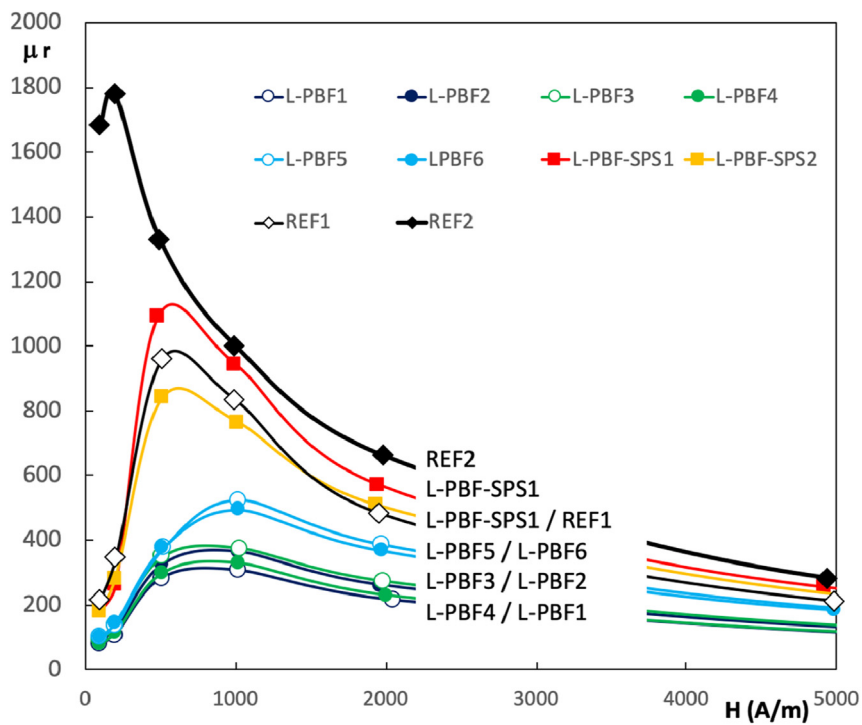
Fig. 8 – Relative permeability versus magnetic field strength. These anhysteretic magnetization curves are obtained with a low excitation frequency (3 Hz) and for various excitation amplitudes.
