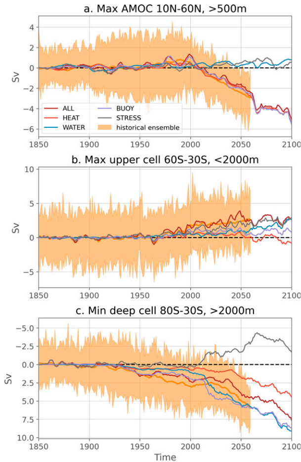
FIG. 6. Time series of circulation anomalies. (a) AMOC (maximum of the Atlantic meridional streamfunction between 10° and 60°N, below 500 m). (b) Southern Ocean upper cell (maximum of the global meridional streamfunction between 30° and 60°S above 2000 m). (c) Southern Ocean deep cell (minimum of the global meridional streamfunction between 30° and 80°S below 2000 m). We take the minimum as the deep cell turns anticlockwise, so has a negative sign. A positive anomaly thus means a decrease in the deep cell, so the y axis is reversed.) In the ocean-only simulations (colored lines) the anomalies are relative to the CTL experiment, with a 5-yr running mean applied for visual purposes. The anomalies in the large ensemble (orange shading) are expressed relative to 1850–99.
