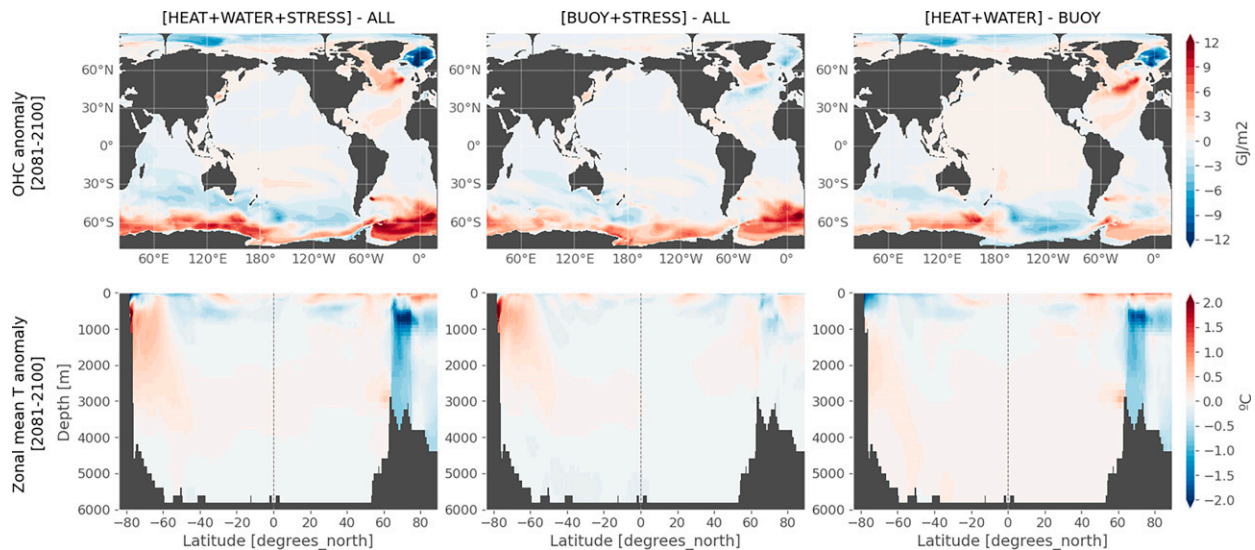
FIG. A1. Differences (left) between the ALL experiment and the sum of HEAT, WATER, and STRESS experiments, (center) between ALL and the sum of BUOY and STRESS, and (right) between BUOY and the sum of HEAT and WATER for ocean heat content and zonal mean temperature anomaly in (2081–2100) relative to the CTL.
