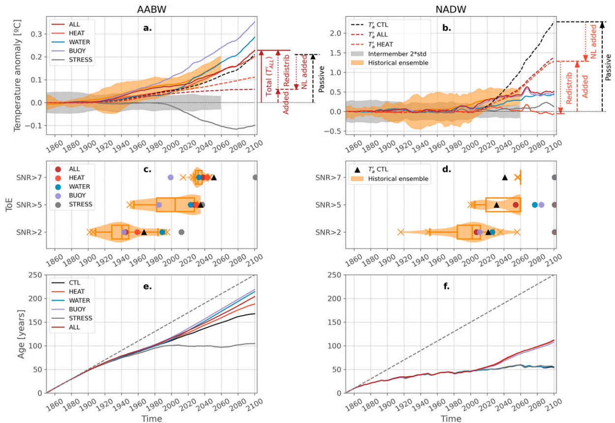
FIG. 8. (a)–(d) As in Fig. 7, but for AABW and NADW. (e),(f) Age tracer in the ocean-only experiments. The gray dotted line represents the values of no ventilation.
