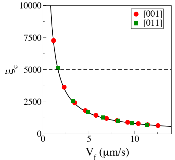
FIG. 5: Convergence scale parameter \xi_c as a function of the facet normal velocity V_f for the two crystal orientations [001] and [011]. For a given V_f , converged results are expected for \xi values below the curve.
