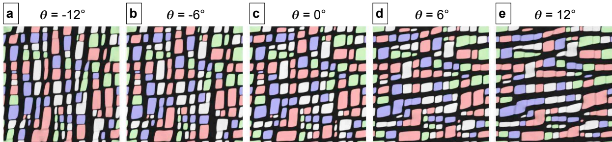
Figure 4: Microstructures obtained at t = 7.6 h with an inhomogenous elasto-viscoplastic simulation for several misorientations \theta of the loading axis a) -12^\circ , b) -6^\circ , c) 0^\circ , d) +6^\circ , e) +12^\circ .
