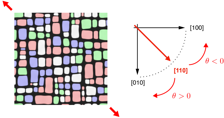
Figure 3: Left: Initial microstructure (colors indicate \gamma' variants) in 4.6^2 \mu\text{m}^2 periodic box. Red arrows represent the applied stress for the perfect [110] crystal orientation. Right: Diagram of the different misorientations applied to the microstructure.
