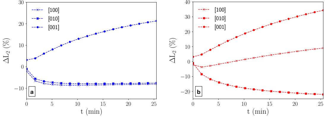
Figure 2: Evolution of \Delta L_2(t) = (L_2(t) - L^0)/L^0 in the three cubic directions for the a - [110] and b - [110]+12 applied load.
