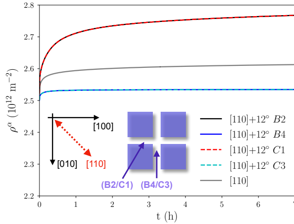
Figure 6: Time evolution of the dislocation densities \rho^\alpha for different directions of the applied load.
