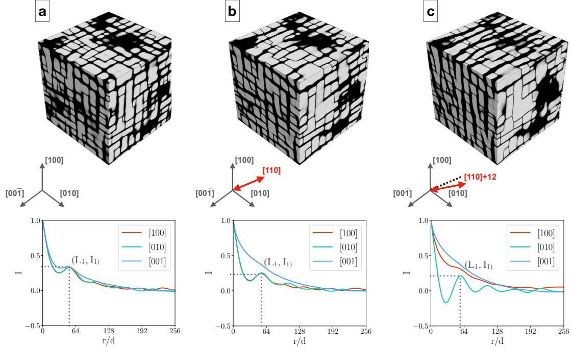
Figure 1: Top: concentration maps of a - the initial cuboidal microstructure and the microstructure obtained with the full elasto-viscoplastic model after t = 25.5 min under b - [110] and c - [110]+12 tensile creep loading. Bottom: corresponding autocorrelation along the cubic axis.
