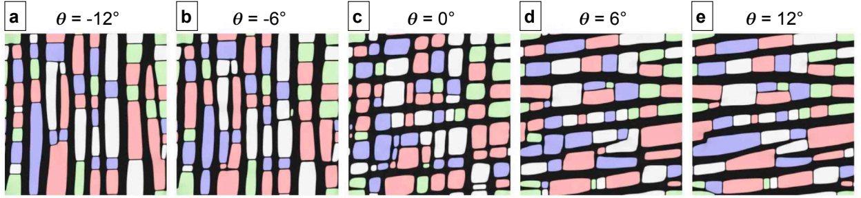
Figure 5: Microstructures obtained at t = 7.6 h with an inhomogeneous elastic simulation with no plasticity for several misorientations \theta of the loading axis a) -12^\circ , b) -6^\circ , c) 0^\circ , d) +6^\circ , e) +12^\circ .
