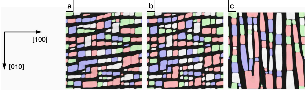
Figure 7: Snapshots of the microstructure in a 4.6^2 \mu\text{m}^2 periodic box after t = 7.6 \text{ h} under [110]+12^\circ creep load in: a - the homogeneous elasto-viscoplastic case, b - the switched elastic constants inhomogeneous elasto-viscoplastic case and c - the switched elastic constants inhomogeneous elastic case.
