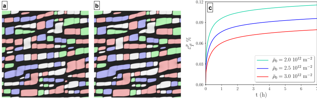
Figure 9: Snapshots of the final microstructure after t = 7.6 \text{ h} under [110]+12^\circ creep load: a - \bar{\rho}_0 = 2.0 \cdot 10^{12} \text{ m}^{-2} and b - 3.0 \cdot 10^{12} \text{ m}^{-2} ; c - corresponding evolution of the average plastic strain \varepsilon_T^P .
