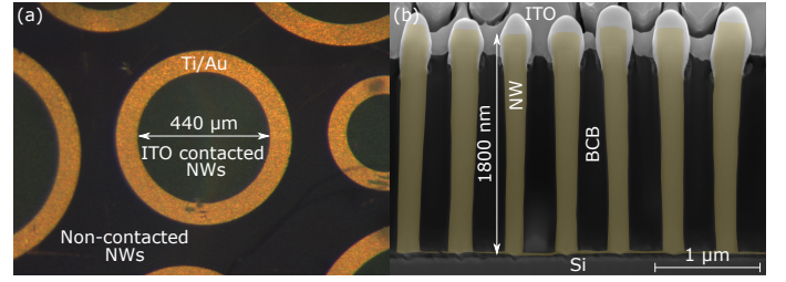
Figure 2 (a) Top view stereo microscope image of the NW solar cell presented in this study. (b) Tilted (45°) SEM image of the same cell, showing its different layers. The as-grown NWs are colored in yellow, while the Si substrate, BCB matrix and ITO are uncolored and can be easily distinguished.
