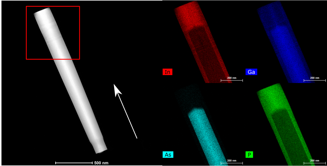
Figure 6 (left) Scanning transmission electron microscopy (STEM) image taken with a high-angle annular dark field (HAADF) detector. The white arrow indicates the GaAs [111]B growth direction. (right) Corresponding In, Ga, As, and P elemental maps of the final NW section, indicated by the red square in the STEM-HAADF image, obtained by energy dispersive X-ray analysis (EDX). The core-shell heterostructure can be seen from the \langle 11\bar{2} \rangle zone-axis.
