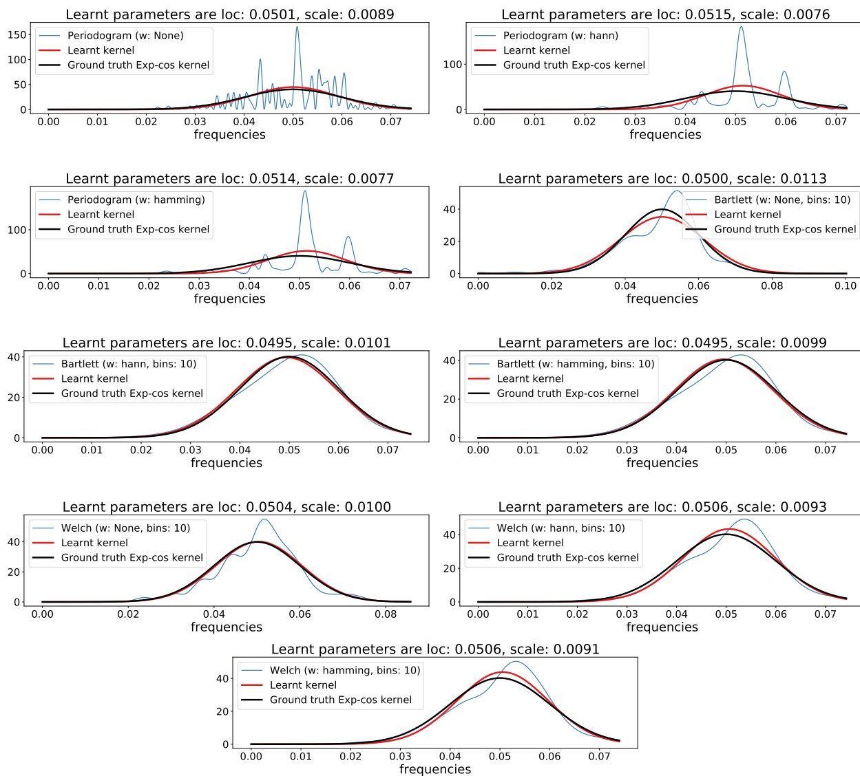
Figure 9: Kernel: Exp-cos.
