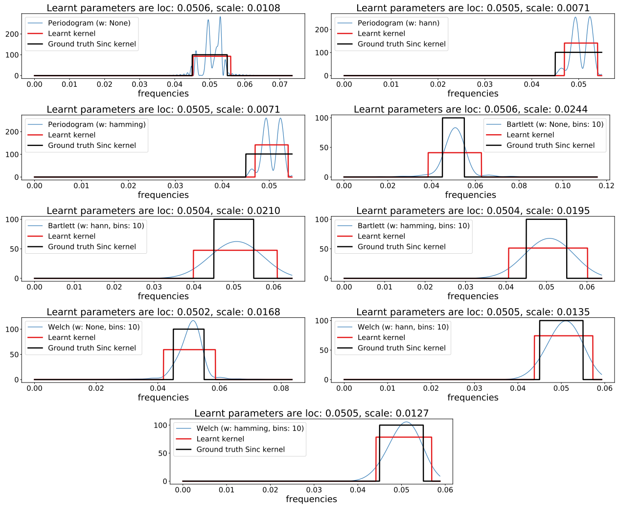
Figure 10: Kernel: Sinc.
