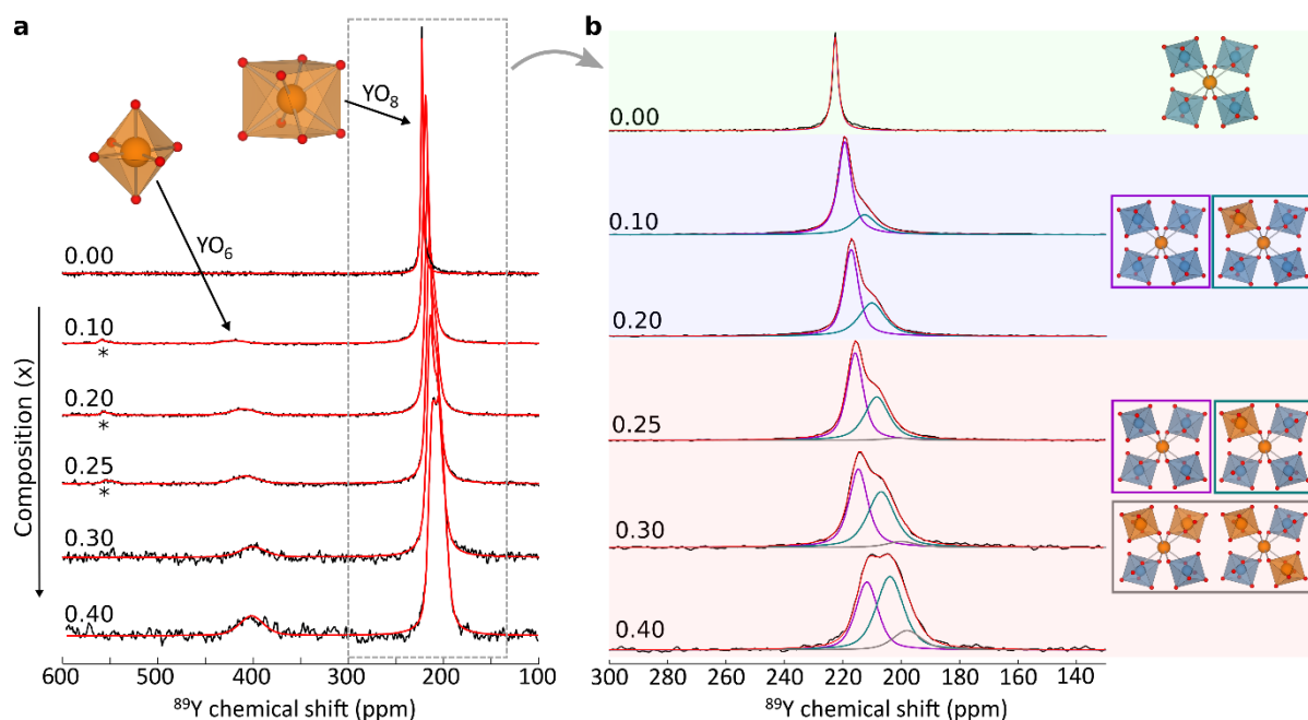
Figure 4. Local structural response to Y^{3+} substitution at the B site in Y_{3+x}Al_{5-x}O_{12} . (a) ^{89}Y NMR spectra showing the emergence of a new resonance above 400 ppm due to YO_6 , whose intensity increases with x . This induces additional components in the YO_8 resonance at 220 ppm from the presence of zero, one or two YO_6 units in its nearest-neighbour sphere, as illustrated in panel (b), where black line = data, red line = overall fit, violet component = zero YO_6 neighbours, green component = one YO_6 , grey component = two YO_6 . All samples are doped with 0.1 mol% Gd^{3+} to reduce ^{89}Y longitudinal relaxation time (see Methods ). Asterisks (*) indicate spinning side bands.
