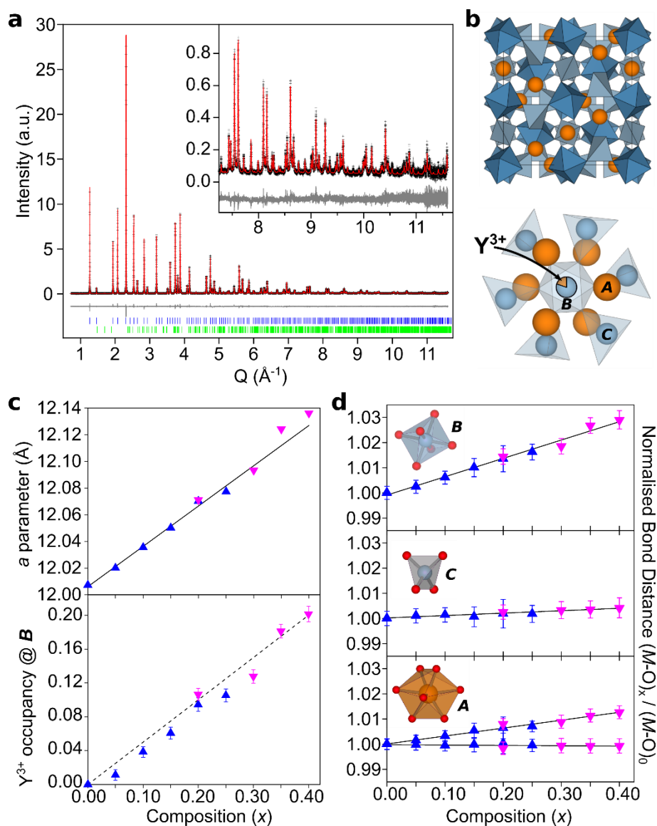
Figure 2. Structural evolution of \text{Y}_{3+x}\text{Al}_{5-x}\text{O}_{12} ( 0 \leq x \leq 0.4 ) from Rietveld analysis of SXRD data. (a) Rietveld refinement of \text{Y}_{3.4}\text{Al}_{4.6}\text{O}_{12} ( R_{wp} = 8.79\% , \chi = 1.16 ) with zoom of the high angle fit inset. Blue tick marks indicate garnet reflections (99.77(2) wt.%), green tick marks indicate perovskite reflections ( \text{YAlO}_3 , 0.33(2) wt.%) (b) The garnet structure of \text{Y}_{3.4}\text{Al}_{4.6}\text{O}_{12} projected along (100), and a fragment projected along (111) showing the three different cation environments A, B and C (orange atoms = \text{Y}^{3+} ; dark blue octahedra = \text{AlO}_6 ; light blue tetrahedra = \text{AlO}_4 ). (c) Refined lattice parameter a with linear fit overlaid (solid line), and refined occupancy of the B site by \text{Y}^{3+} with nominal occupancy overlaid (dashed line). (d) Refined metal-oxygen distances (M\text{-O})_x in the three different cation environments, normalised to their values at \text{Y}_3\text{Al}_5\text{O}_{12} (M\text{-O})_0 . Blue triangles = direct crystallised samples; magenta inverted triangles = glass crystallised samples. Error bars correspond to 10x esd from the refinements.
