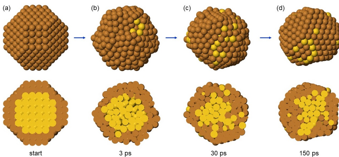
Fig. 9 Snapshots from the initial part of a simulation of \text{Au}_{140}\text{Cu}_{446} at T = 600 K. In the top row, the cluster surface is shown, while in the bottom row, cross sections are given to show the degree of intermixing. Cu and Au atoms are coloured in brownish and yellow, respectively.
