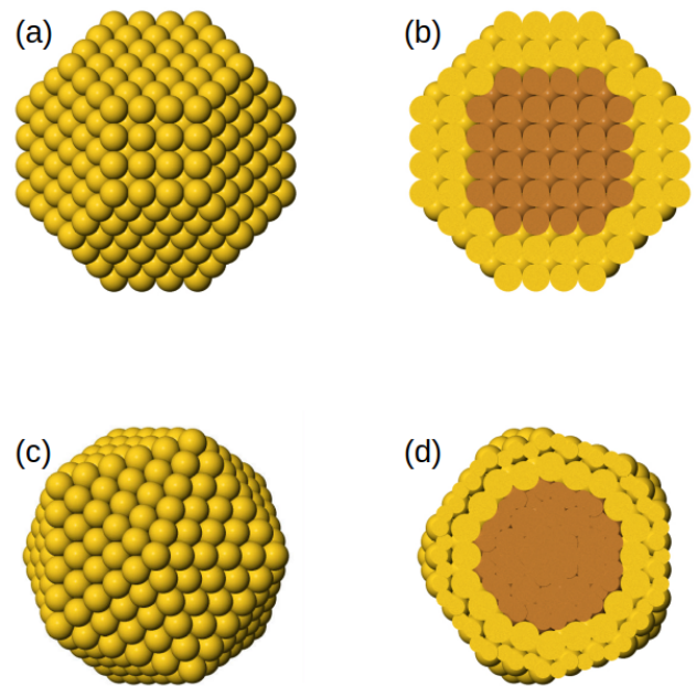
Fig. 1 (a-b) Initial truncated octahedral structure of 586 atoms with core@shell chemical ordering: (a) shows its surface, whereas (b) shows a cross section. (c-d) Initial icosahedral structure of 561 atoms with core@shell chemical ordering: (c) shows its surface, whereas (d) shows a cross section.
