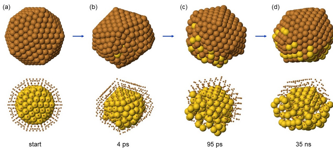
Fig. 8 Snapshots from the initial part of a simulation of \text{Au}_{147}\text{Cu}_{414} at T = 600 K. In the top row, the cluster surface is shown, while in the bottom row, Cu atoms (brownish) are displayed as small spheres to show the structure of the Au core (in yellow).
