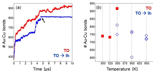
Fig. 7 (a) Time dependence of the number of Au-Cu bonds in two simulations starting from a Cu@Au TO of composition \text{Au}_{446}\text{Cu}_{140} . Simulation temperature is 550 K. In the first simulation (red curve) the structure remains in the TO motif till the end, while in the second simulation (blue curve) a TO→Ih transformation takes place between 4 and 5 \mu\text{s} . The black arrow indicates the moment at which the transformation occurs, which corresponds to a meaningful change in the time evolution of the mixed bonds. (b) Final number (averaged over the last \mu\text{s} of the simulation) of nearest neighbour Au-Cu bonds. Red squares correspond to simulations in which the structure remains in the TO motif, whereas blue diamonds correspond to simulations in which the TO→Ih transformation takes place at some stage. Note that more than 1000 Au-Cu nearest-neighbour bonds are expected at equilibrium (see Fig. 6(a)), a value which is significantly larger than those of the MD simulations.
