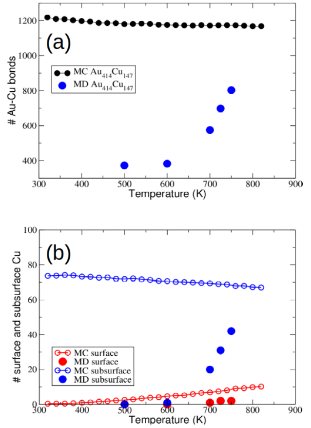
Fig. 6 Simulation results for the Au 414 Cu 147 Ih structure. (a) Comparison between the number of Au-Cu neighbour bonds at equilibrium (MC data) and at the end of the MD simulations. (b) Comparison between equilibrium MC and MD data for the number of surface and subsurface atoms. The MD data are averaged over the last \mu s of the simulations.
