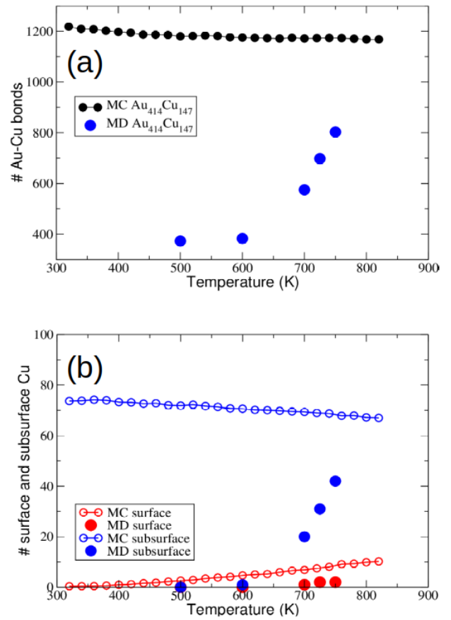
Fig. 6 Simulation results for the Au 414 Cu 147 Ih structure. (a) Comparison between the number of Au-Cu nearest neighbour bonds at equilibrium (MC data) and at the end of the MD simulations. (b) Comparison between equilibrium MC and MD data for the number of surface and subsurface atoms. The MD data are averaged over the last \mu s of the simulations.
