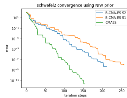
Figure 7: Convergence for the Schwefel 2 function
