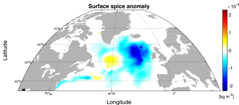
Fig. 21 Surface spice anomaly [ \text{kg m}^{-3} ] 2 years after the freshening of the Labrador Sea (Experiment Pert1_LabSSS)
