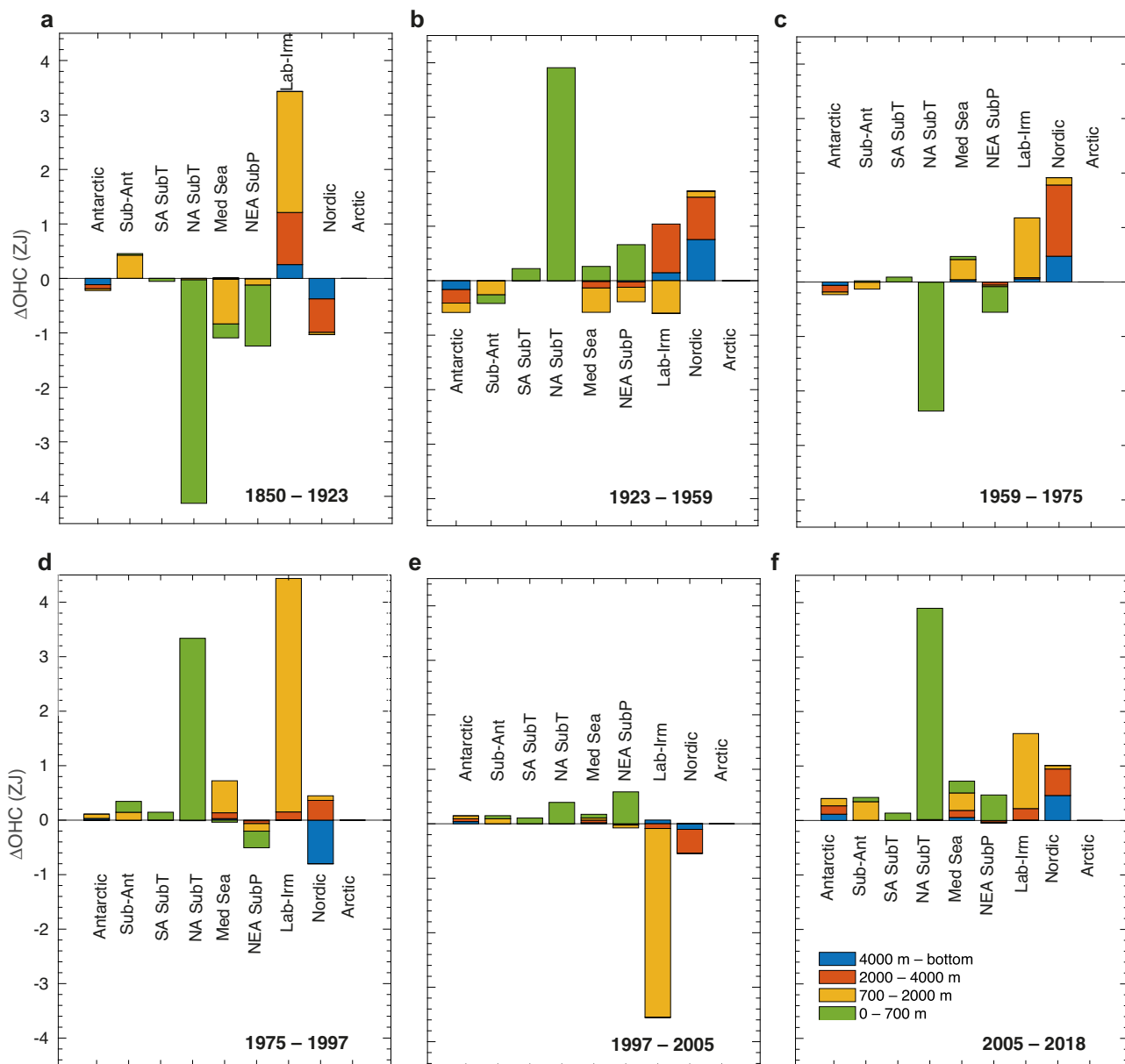
Fig. 5 Regional heat uptake contributions to 25°N \Delta OHC for six time intervals. Same as Fig. 3 but for excess heat contributions (ZJ) from the source regions for different time intervals at 25°N, which we observed, have shaped the 0-700 m \Delta OHC: (a) 1850-1923, (b) 1923-1959, (c) 1959-1975 (d) 1975-1997, (e) 1997-2005, and (f) 2005-2018.
