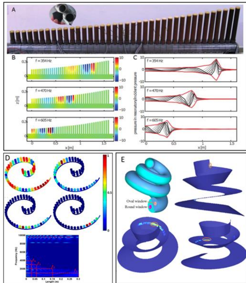
Figure 14 : Metamaterial inspired by the cochlea. Some of the examples of cochlea-inspired for the design of metamaterials. In particular, in panels A,B,C, a gradient-index metamaterial for airborne sounds, made from 38 quarter-wavelength acoustic resonators of different heights is reproduced (adapted from [202]). In panel D, a rainbow trapper based on a set of Helmholtz resonators is described (adapted from [205]). In panel E, a modal analysis of a helix model of cochlea is reported, showing a different response to different frequency excitations.
