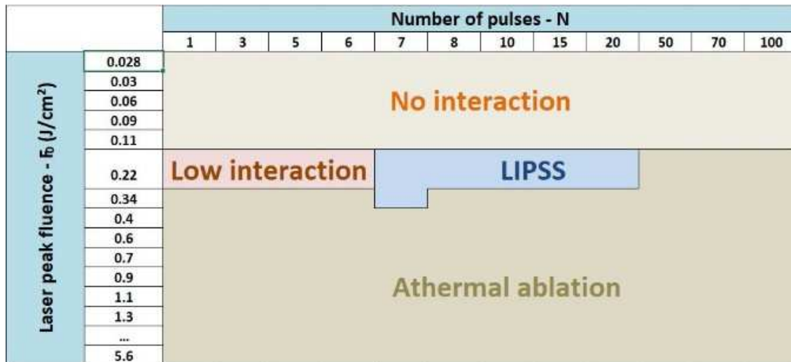
Fig. 9. Laser-matter interaction domain map for tungsten carbide.
