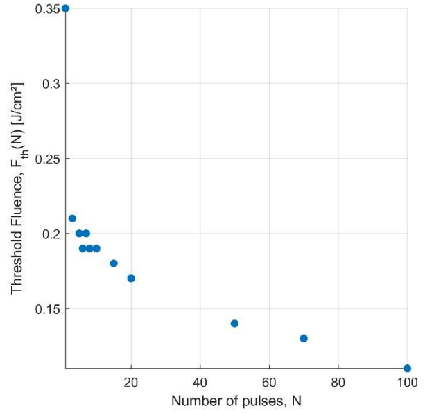
Fig. 3. Threshold fluence as a function of number of pulses.
