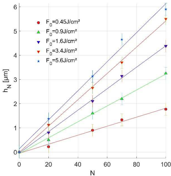
Fig. 6. Ablation depth h_N versus the number of pulses N for F_0 = 0.45, 0.9, 1.6, 3.4, 5.6 \text{ J/cm}^2
