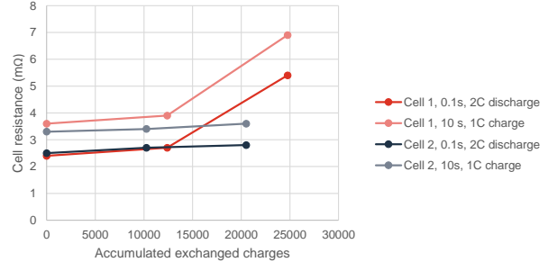
Fig. 5: Evolution of the internal resistance of cell 1 and 2, at two different conditions
