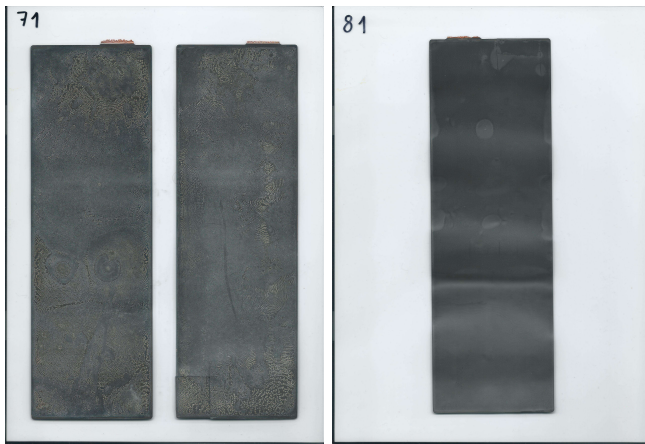
Fig. 7: Scan of the anodes of cell 1 (left) and cell 2 (right)
