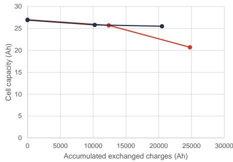
Fig. 4: Measurement of both cells capacity
