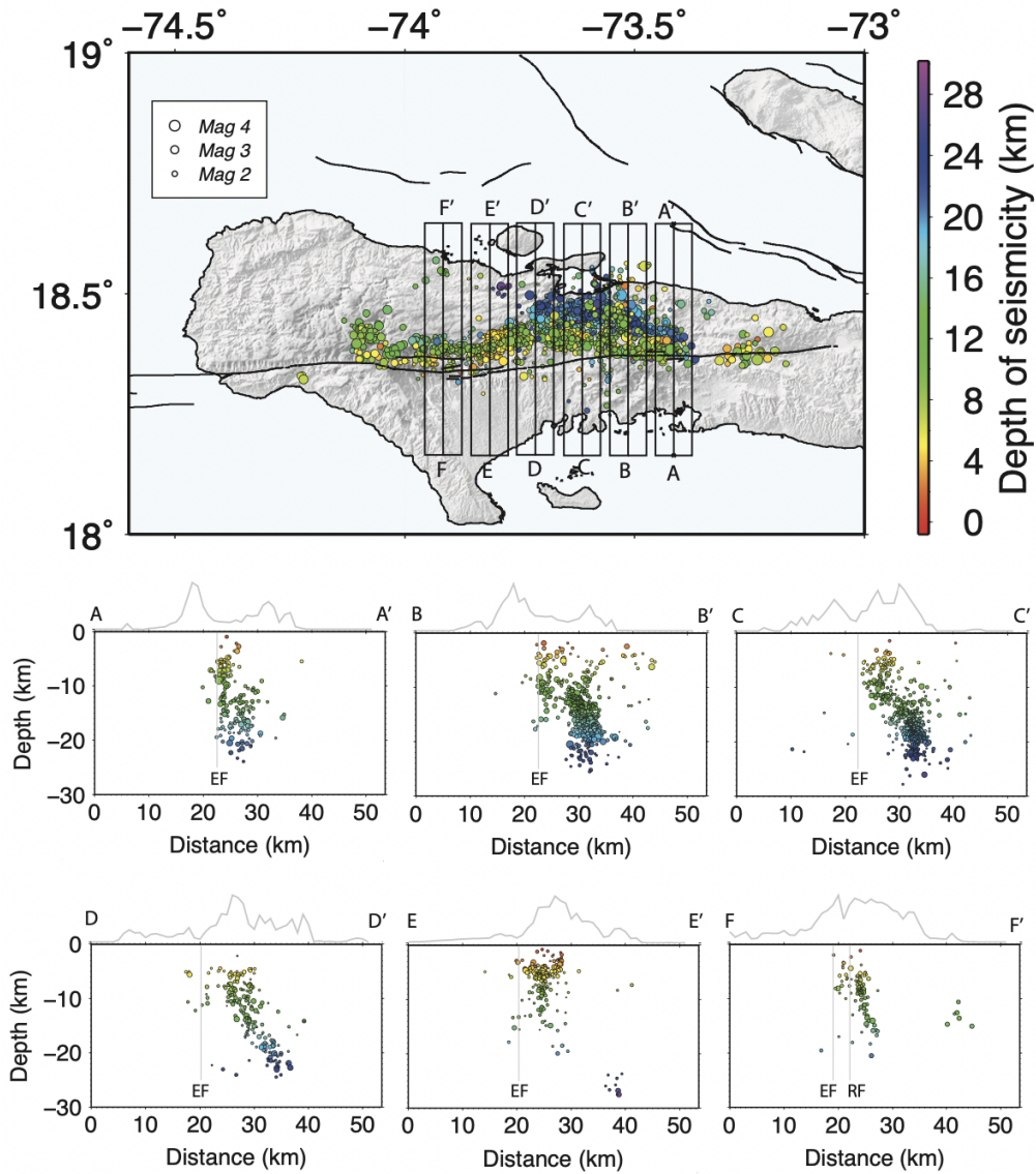
Figure 11: North-South cross sections illustrating the correlation of the fault structures with respect to the EPG fault. Hypocenters within the rectangular box are projected into the corresponding cross sections. Gray curve above each cross section indicates the surface topography. The vertical gray lines mark the location of either the EPG fault (EF) or the Ravine du Sud fault (RF).
