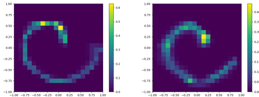
Fig. 4. Regularizers learned via the proposed method with different learning parameters. Using the same number of grid points, we have better result when the network has more neurons. (Left) 3 hidden layers with 64, 128, 256 neurons in each layer. (Right) 3 hidden layers with 64, 128, 192 neurons in each layer.
