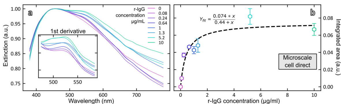
Figure 6. (a) Normalized and smoothed extinction spectra of immunocomplex suspensions resulting from the addition of rabbit IgG in the range 0–10 \mu\text{g/mL} ; (b) Dose–response curve plotted from the integrated area of the first order derivative spectra between 475 and 585 nm vs. rabbit IgG concentration.
