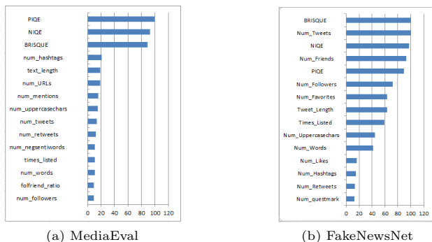
Fig. 5 Random Forest feature importance
