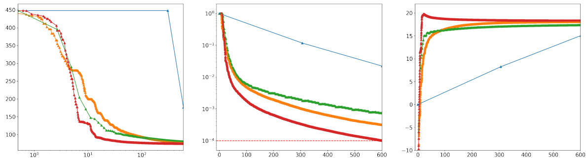
Figure 2: Evolution of quantitative metrics along time (in seconds), for algorithms 3MG (blue), ABGD (orange), BP3MG (green) and BD3MG (red), for FlyBrain restoration. Evolution of \|\mathbf{x}^k - \bar{\mathbf{x}}\| (left), \|\mathbf{x}^{k+1} - \mathbf{x}^k\|/\|\mathbf{x}^k\| (middle), and SNR in dB (right).
