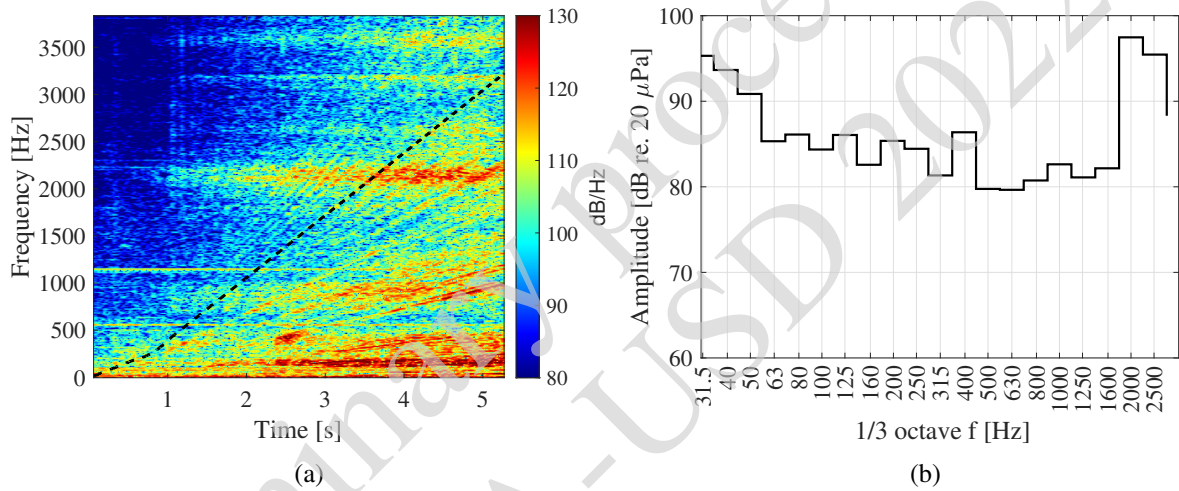
Figure 5: Order analysis of reference microphone signal: (a) Spectrogram with order 79.5 (---) highlighted and (b) Order 79.5 presented in third-octave band.
