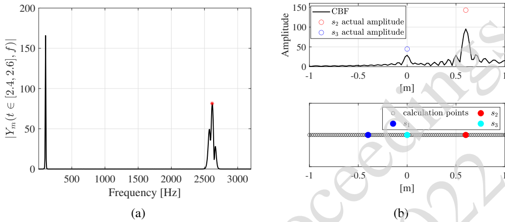
Figure 2: Solution with conventional beamforming: (a) spectrum of an array microphone with df = 5 Hz; red star denotes 2615 Hz and (b) CBF source map at 2615 Hz.
